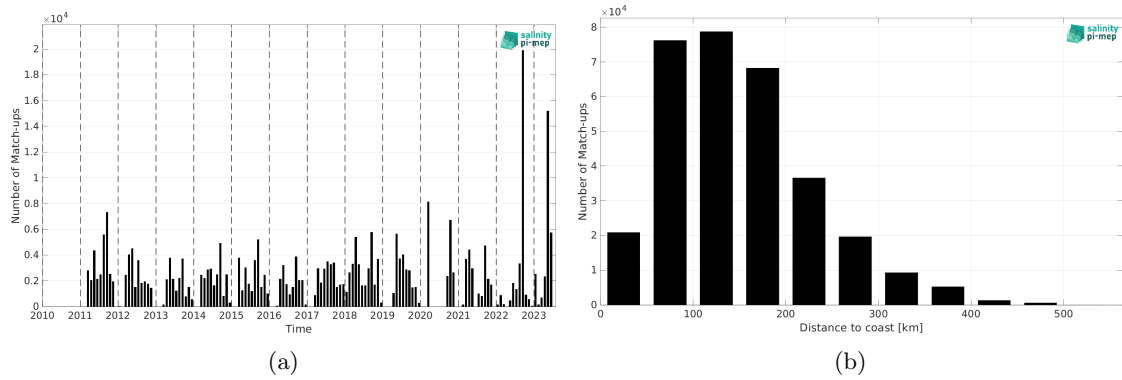
Figure 1: Number of match-ups between TSG (SAMOS) and SMOS SSS L4 OI v342 - Weekly (CMEMS-CATDS-LOPS) SSS as a function of time (a) and as function of the distance to coast (b) over the Mississippi river plume Pi-MEP region and for the full satellite product period.
