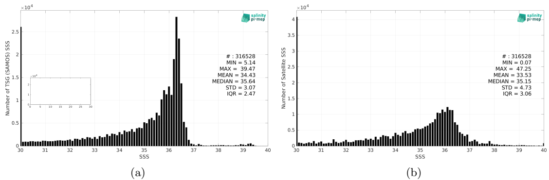
Figure 2: Histograms of SSS from TSG (SAMOS) (a) and SMOS SSS L4 OI v342 - Weekly (CMEMS-CATDS-LOPS) (b) considering all match-up pairs per bins of 0.1 over the Mississippi river plume Pi-MEP region and for the full satellite product period.
