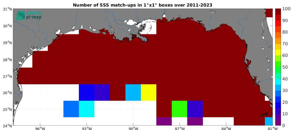
Figure 4: Number of SSS match-ups between TSG (SAMOS) SSS and the SMOS SSS L4 OI v342 - Weekly (CMEMS-CATDS-LOPS) SSS product for the Mississippi river plume Pi-MEP region over 1^\circ \times 1^\circ boxes and for the full satellite product period.
