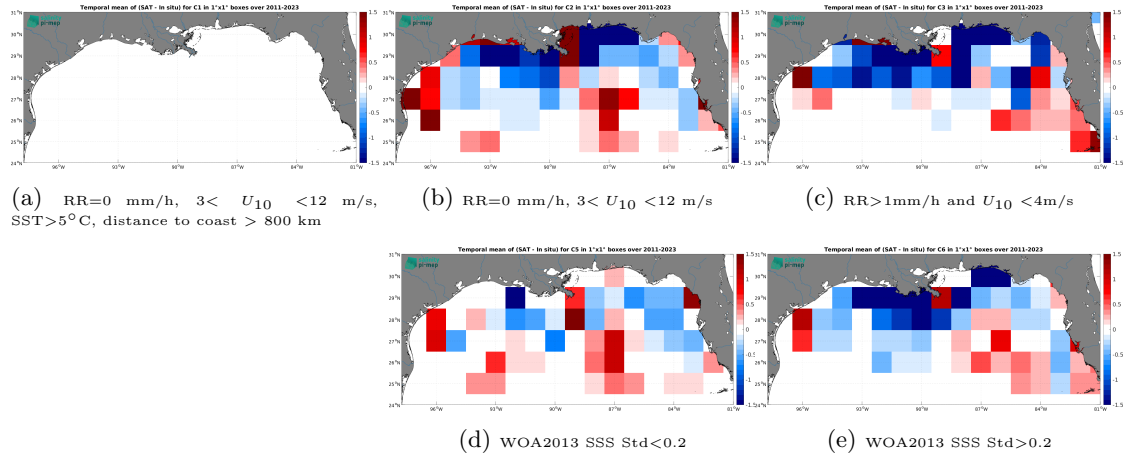
Figure 12: Temporal mean gridded over spatial boxes of size 1^{\circ}\times 1^{\circ} of \Delta\text{SSS} (SMOS SSS L4 OI v342 - Weekly (CMEMS-CATDS-LOPS) - TSG (SAMOS)) for 5 different subdatasets corresponding to:RR=0 mm/h, 3 < U_{10} < 12 m/s, SST >5^{\circ}\text{C} , distance to coast > 800 km (a), RR=0 mm/h, 3 < U_{10} < 12 m/s (b), RR >1 mm/h and U_{10} < 4 m/s (c), WOA2013 SSS Std <0.2 (d), WOA2013 SSS Std >0.2 (e).
