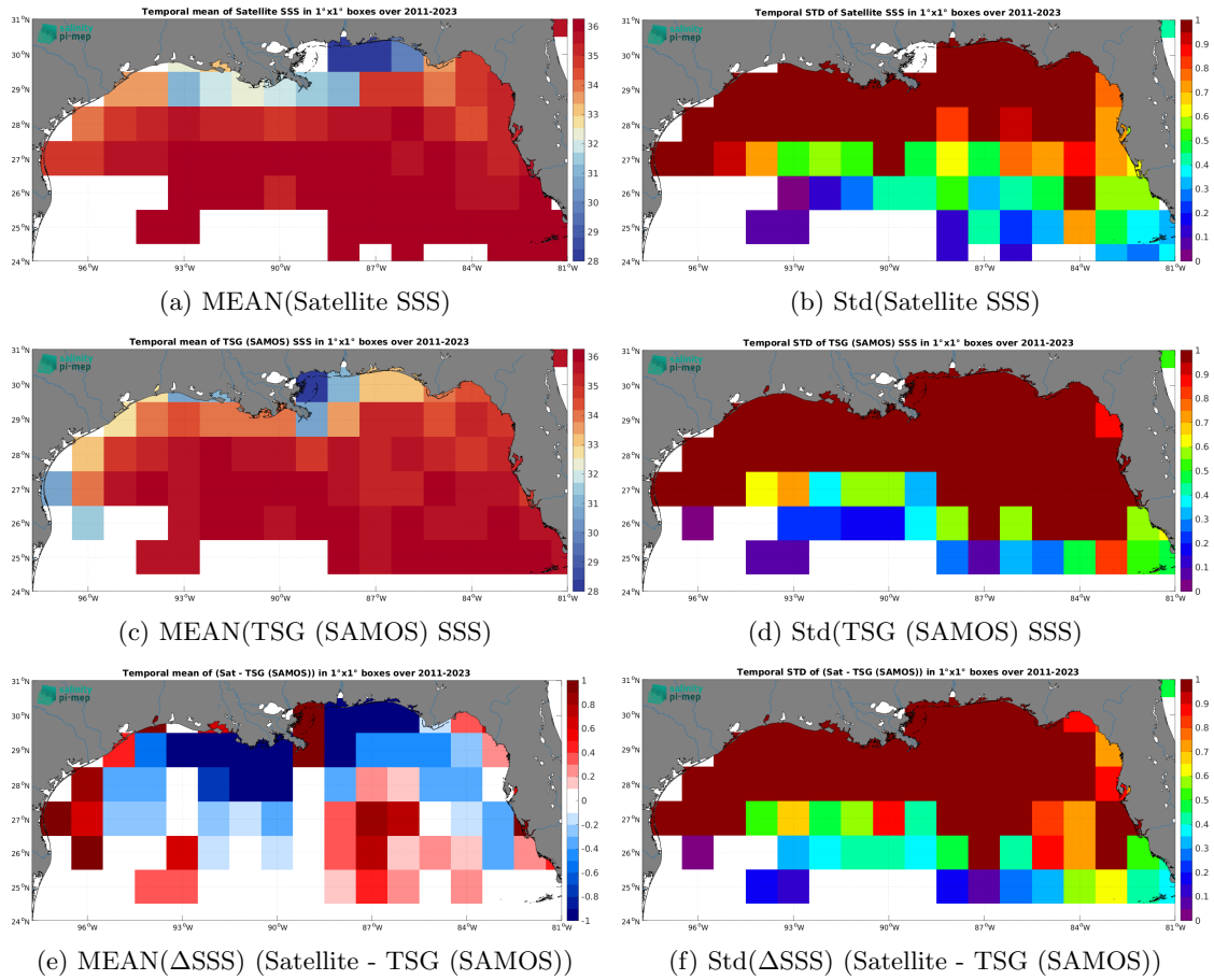
Figure 6: Temporal mean (left) and Std (right) of SSS from SMOS SSS L4 OI v342 - Weekly (CMEMS-CATDS-LOPS) (top), TSG (SAMOS) (middle), and of \Delta SSS (Satellite - TSG (SAMOS)). Only match-up pairs are used to generate these maps.
