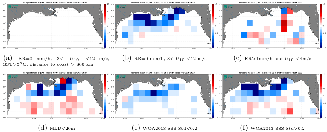
Figure 12: Temporal mean gridded over spatial boxes of size 1^{\circ}\times 1^{\circ} of \Delta\text{SSS} (SMOS SSS L4 OI v342 - Weekly (CMEMS-CATDS-LOPS) - Argo) for 6 different subdatasets corresponding to:RR=0 mm/h, 3 < U_{10} < 12 m/s, SST > 5^{\circ}\text{C} , distance to coast > 800 km (a), RR=0 mm/h, 3 < U_{10} < 12 m/s (b), RR > 1\text{mm/h} and U_{10} < 4\text{m/s} (c),MLD < 20\text{m} (d),WOA2013 SSS Std < 0.2 (e),WOA2013 SSS Std > 0.2 (f).
