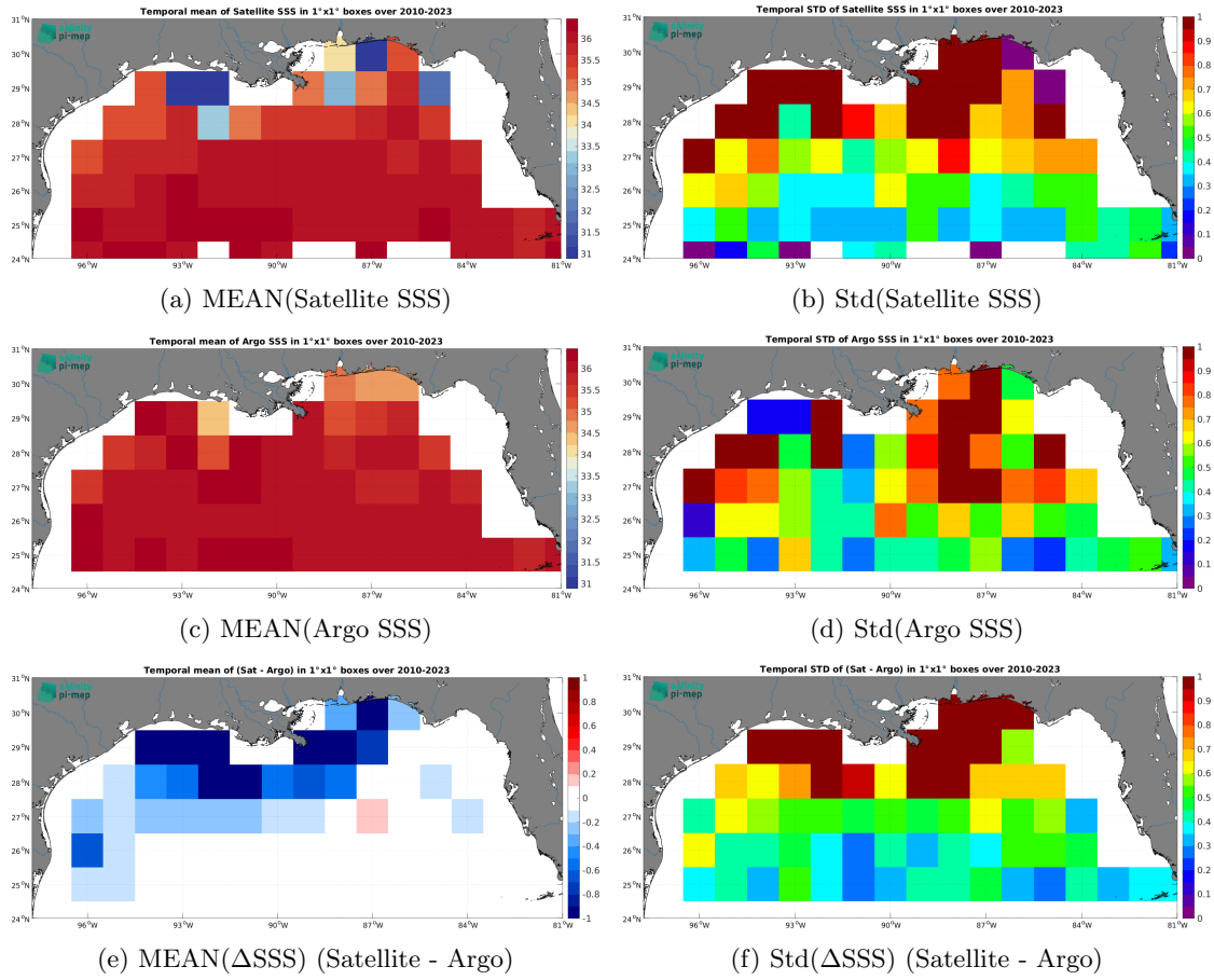
Figure 6: Temporal mean (left) and Std (right) of SSS from SMOS SSS L4 OI v342 - Weekly (CMEMS-CATDS-LOPS) (top), Argo (middle), and of \Delta SSS (Satellite - Argo). Only match-up pairs are used to generate these maps.
