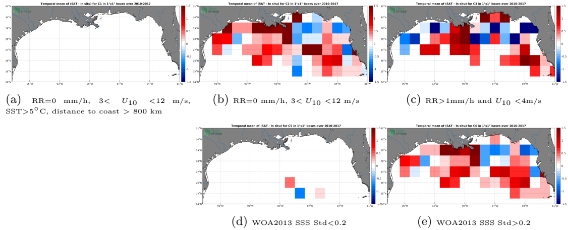
Figure 12: Temporal mean gridded over spatial boxes of size 1^{\circ}\times 1^{\circ} of \Delta\text{SSS} (SMOS-L4-CATDS-CECOS-IFREMER-V2-WEEKLY-0.5DEG - TSG-SAMOS) for 5 different subdatasets corresponding to:RR=0 mm/h, 3 < U_{10} < 12 m/s, SST >5^{\circ}\text{C} , distance to coast > 800 km (a), RR=0 mm/h, 3 < U_{10} < 12 m/s (b), RR >1 mm/h and U_{10} < 4 m/s (c), WOA2013 SSS Std <0.2 (d), WOA2013 SSS Std >0.2 (e).
