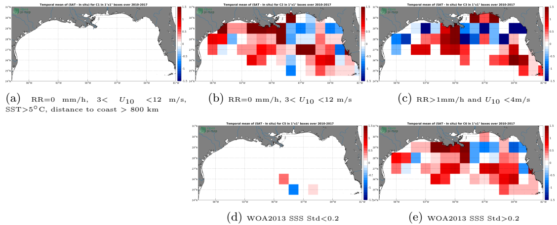
Figure 12: Temporal mean gridded over spatial boxes of size 1^\circ \times 1^\circ of \Delta SSS (SMOS-L4-CATDS-CECOS-IFREMER-V2-WEEKLY-0.5DEG - TSG-SAMOS) for 5 different subdatasets corresponding to: RR=0 mm/h, 3 < U_{10} < 12 m/s, SST > 5^\circ C , distance to coast > 800 km (a), RR=0 mm/h, 3 < U_{10} < 12 m/s (b), RR > 1 mm/h and U_{10} < 4 m/s (c), WOA2013 SSS Std < 0.2 (d), WOA2013 SSS Std > 0.2 (e).
