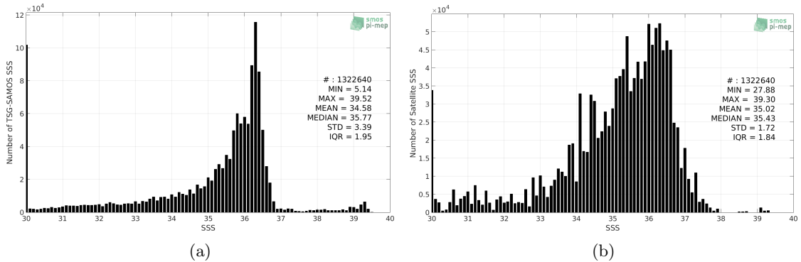
Figure 2: Histograms of SSS from TSG-SAMOS (a) and SMOS-L4-CATDS-CECOS-IFREMER-V2-WEEKLY-0.5DEG (b) considering all match-up pairs per bins of 0.1 over the Mississippi river plume Pi-MEP region and for the full satellite product period.
