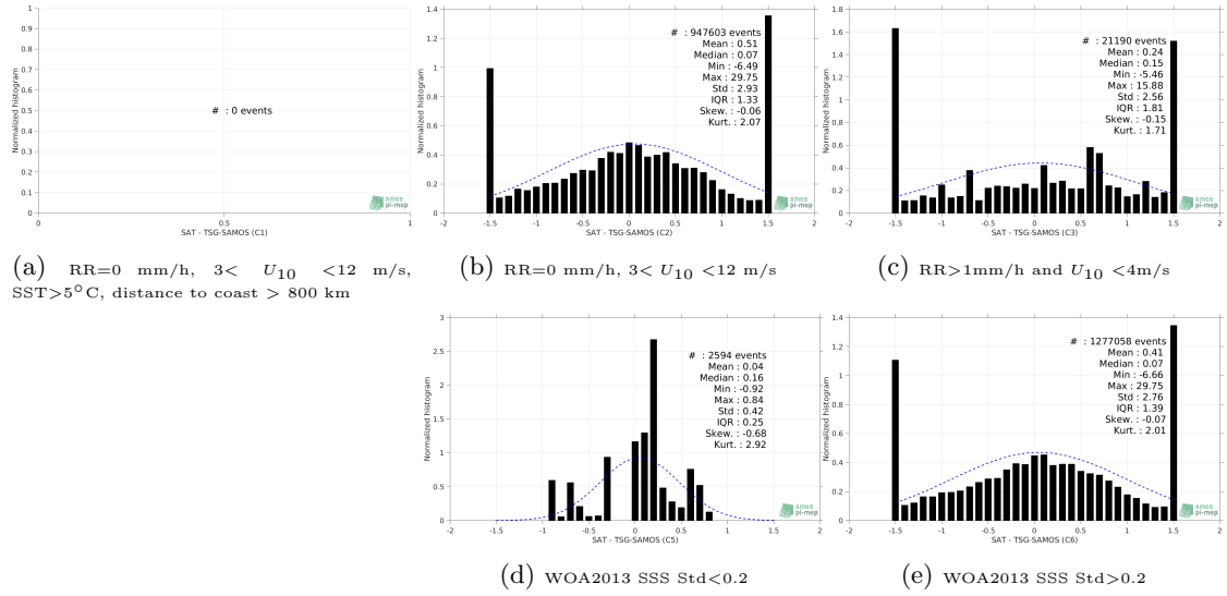
Figure 13: Normalized histogram of \Delta SSS (SMOS-L4-CATDS-CECOS-IFREMER-V2-WEEKLY-0.5DEG - TSG-SAMOS) for 5 different subdatasets corresponding to: RR=0 mm/h, 3 < U_{10} < 12 m/s, SST > 5°C, distance to coast > 800 km (a), RR=0 mm/h, 3 < U_{10} < 12 m/s (b), RR > 1mm/h and U_{10} < 4 m/s (c), WOA2013 SSS Std < 0.2 (d), WOA2013 SSS Std > 0.2 (e).
