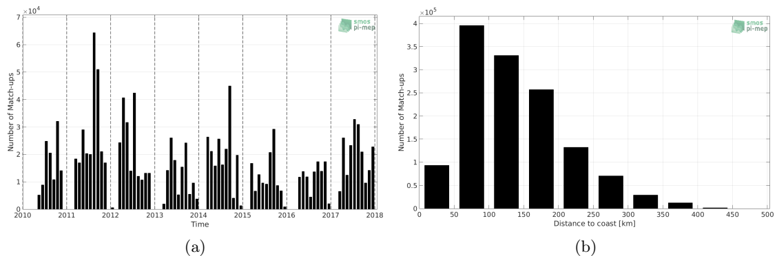
Figure 1: Number of match-ups between TSG-SAMOS and SMOS-L4-CATDS-CECOS-IFREMER-V2-WEEKLY-0.5DEG SSS as a function of time (a) and as function of the distance to coast (b) over the Mississippi river plume Pi-MEP region and for the full satellite product period.
