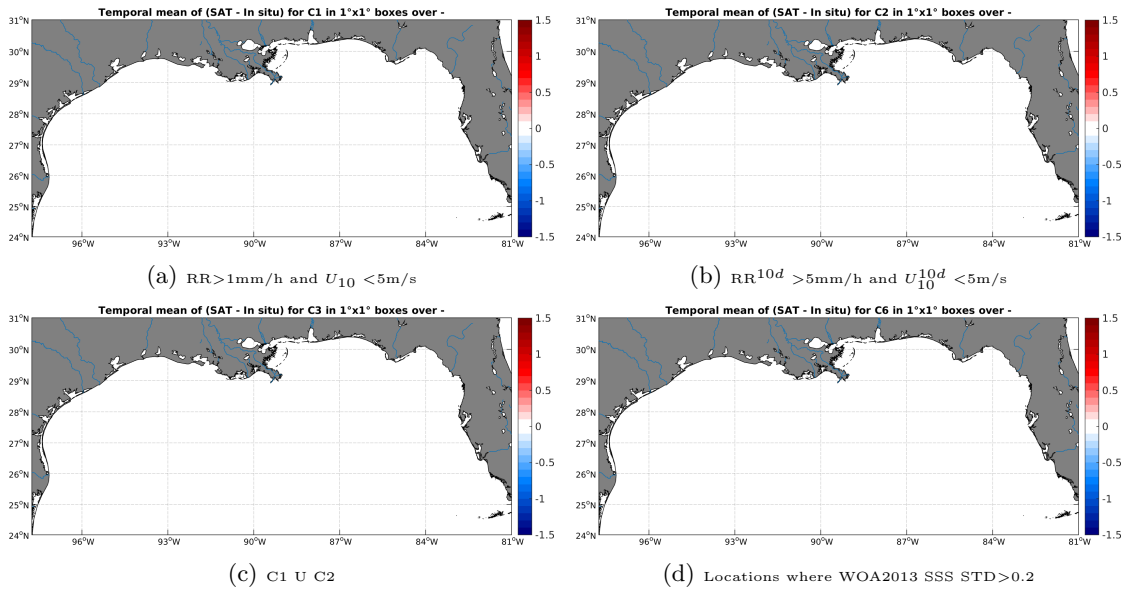
Figure 12: Temporal mean gridded over spatial boxes of size 1^\circ \times 1^\circ of \Delta SSS (SMOS-L4-CATDS-CECOS-IFREMER-V2-WEEKLY-0.5DEG - TSG-LEGOS-DM) for 4 different subdatasets corresponding to: RR > 1\text{mm/h} and U_{10} < 5\text{m/s} (a), RR^{10d} > 5\text{mm/h} and U_{10}^{10d} < 5\text{m/s} (b), C1 U C2 (c), Locations where WOA2013 SSS STD > 0.2 (d).
