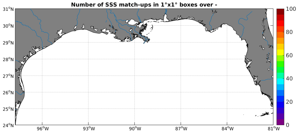
Figure 4: Number of SSS match-ups between TSG-LEGOS-DM SSS and the SMOS-L4-CATDS-CECOS-IFREMER-V2-WEEKLY-0.5DEG SSS product for the Mississippi river plume Pi-MEP region over 1^\circ \times 1^\circ boxes and for the full satellite product period.
