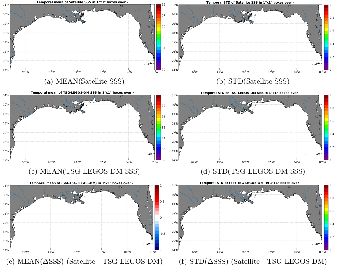
Figure 6: Temporal mean (left) and STD (right) of SSS from SMOS-L4-CATDS-CECOS-IFREMER-V2-WEEKLY-0.5DEG (top), TSG-LEGOS-DM (middle), and of \Delta\text{SSS} (Satellite - TSG-LEGOS-DM). Only match-up pairs are used to generate these maps.
