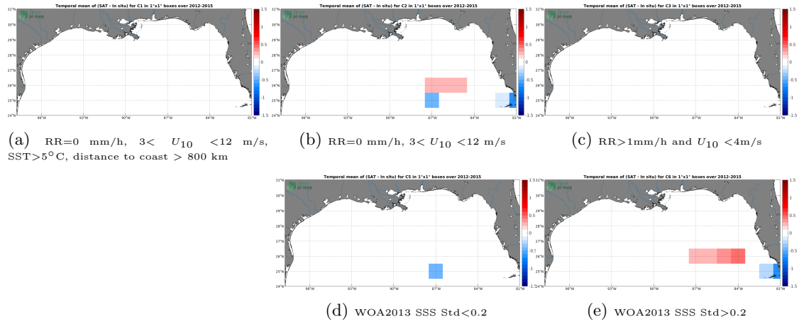
Figure 12: Temporal mean gridded over spatial boxes of size 1^\circ \times 1^\circ of \Delta SSS (SMOS L4 v2 Weekly (CATDS-CECOS-IFREMER) - TSG (GOSUD-Sailing-ship)) for 5 different subdatasets corresponding to: RR=0 mm/h, 3 < U_{10} < 12 m/s, SST > 5^\circ\text{C} , distance to coast > 800 km (a), RR=0 mm/h, 3 < U_{10} < 12 m/s (b), RR > 1 mm/h and U_{10} < 4 m/s (c), WOA2013 SSS Std < 0.2 (d), WOA2013 SSS Std > 0.2 (e).
