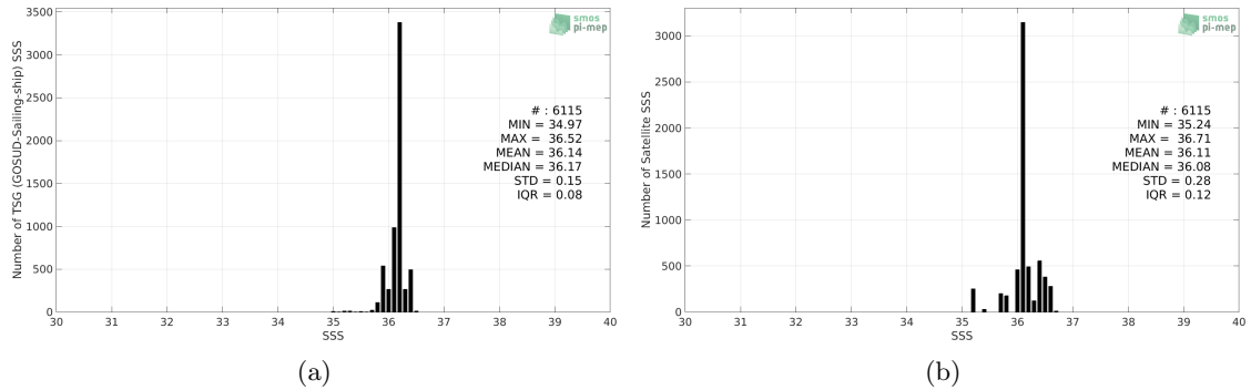
Figure 2: Histograms of SSS from TSG (GOSUD-Sailing-ship) (a) and SMOS L4 v2 Weekly (CATDS-CECOS-IFREMER) (b) considering all match-up pairs per bins of 0.1 over the Mississippi river plume Pi-MEP region and for the full satellite product period.
