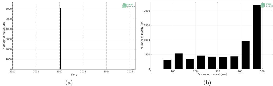
Figure 1: Number of match-ups between TSG (GOSUD-Sailing-ship) and SMOS L4 v2 Weekly (CATDS-CECOS-IFREMER) SSS as a function of time (a) and as function of the distance to coast (b) over the Mississippi river plume Pi-MEP region and for the full satellite product period.
