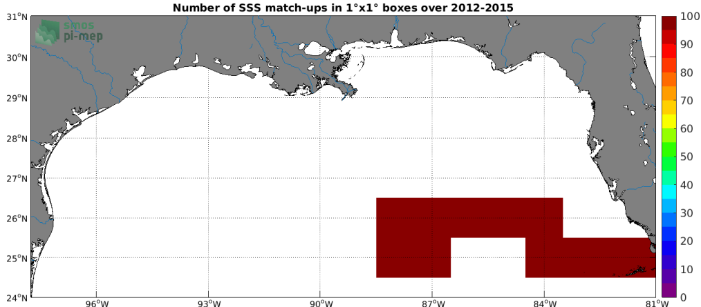
Figure 4: Number of SSS match-ups between TSG (GOSUD-Sailing-ship) SSS and the SMOS L4 v2 Weekly (CATDS-CECOS-IFREMER) SSS product for the Mississippi river plume Pi-MEP region over 1^\circ \times 1^\circ boxes and for the full satellite product period.
