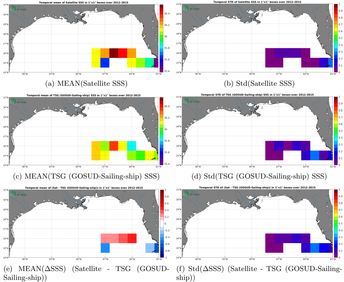
Figure 6: Temporal mean (left) and Std (right) of SSS from SMOS L4 v2 Weekly (CATDS-CECOS-IFREMER) (top), TSG (GOSUD-Sailing-ship) (middle), and of \Delta\text{SSS} (Satellite - TSG (GOSUD-Sailing-ship)). Only match-up pairs are used to generate these maps.
