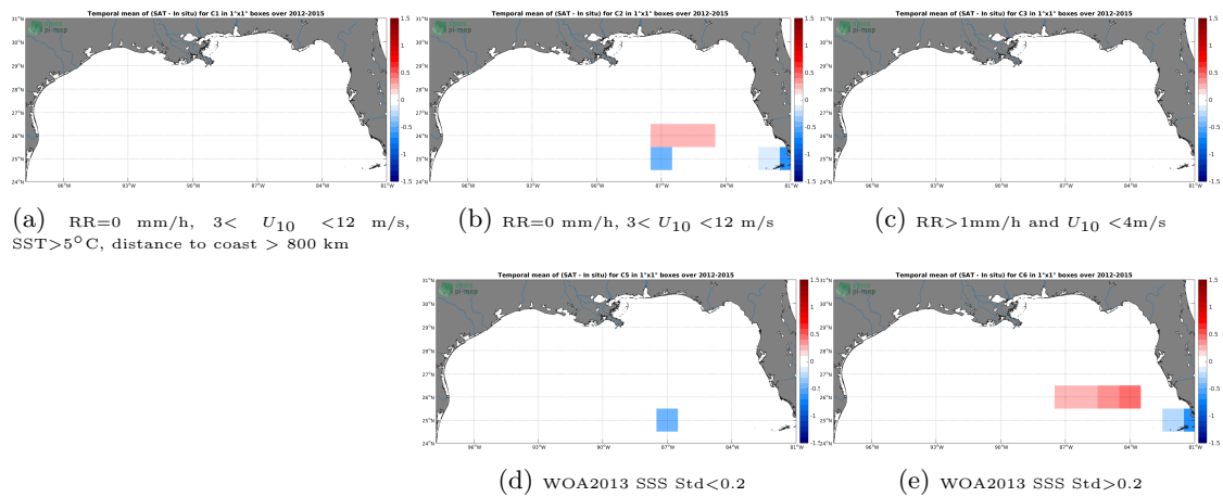
Figure 12: Temporal mean gridded over spatial boxes of size 1^\circ \times 1^\circ of \Delta SSS (SMOS-L4-CATDS-CECOS-IFREMER-V2-WEEKLY-0.5DEG - TSG-GOSUD-Sailing-ship) for 5 different subdatasets corresponding to:RR=0 mm/h, 3 < U_{10} < 12 m/s, SST>5°C, distance to coast > 800 km (a), RR=0 mm/h, 3 < U_{10} < 12 m/s (b), RR>1mm/h and U_{10} < 4 m/s (c), WOA2013 SSS Std<0.2 (d), WOA2013 SSS Std>0.2 (e).
