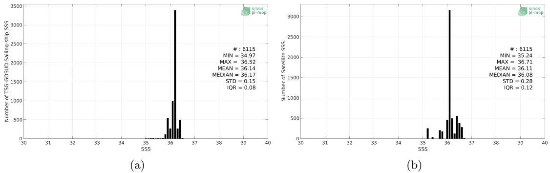
Figure 2: Histograms of SSS from TSG-GOSUD-Sailing-ship (a) and SMOS-L4-CATDS-CECOS-IFREMER-V2-WEEKLY-0.5DEG (b) considering all match-up pairs per bins of 0.1 over the Mississippi river plume Pi-MEP region and for the full satellite product period.
