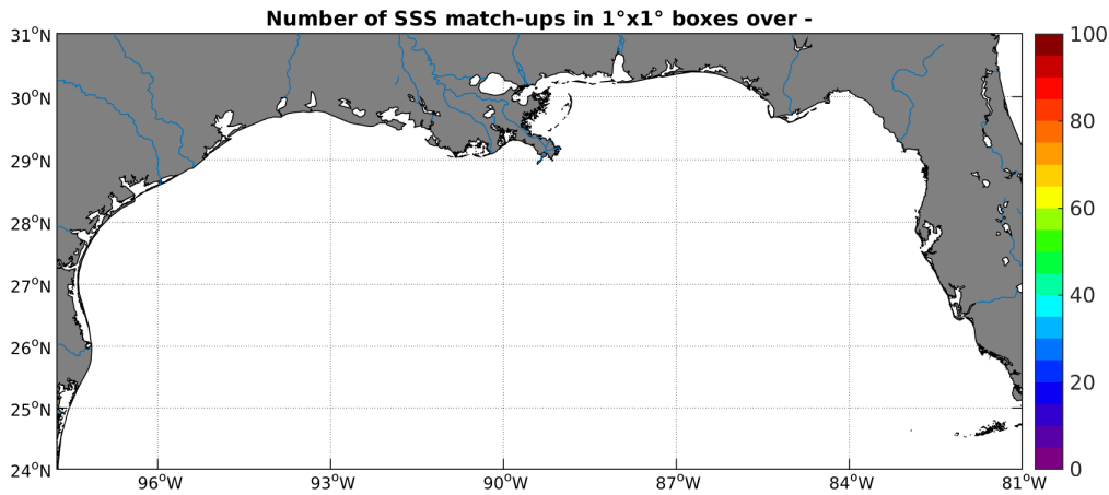
Figure 4: Number of SSS match-ups between TSG-GOSUD-Research-vessel SSS and the SMOS-L4-CATDS-CECOS-IFREMER-V2-WEEKLY-0.5DEG SSS product for the Mississippi river plume Pi-MEP region over 1°x1° boxes and for the full satellite product period.
