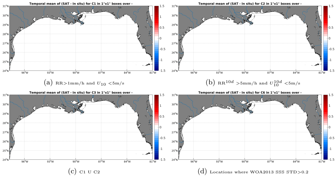
Figure 12: Temporal mean gridded over spatial boxes of size 1^\circ \times 1^\circ of \Delta SSS (SMOS-L4-CATDS-CECOS-IFREMER-V2-WEEKLY-0.5DEG - TSG-GOSUD-Research-vessel) for 4 different sub-datasets corresponding to:RR >1 mm/h and U_{10} < 5 m/s (a), RR ^{10d} > 5 mm/h and U_{10}^{10d} < 5 m/s (b), C1 U C2 (c),Locations where WOA2013 SSS STD >0.2 (d).
