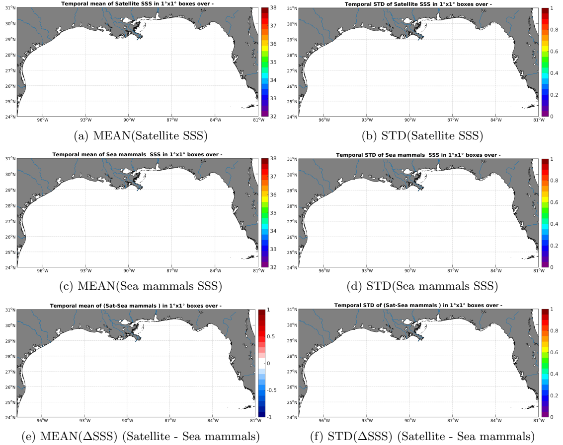
Figure 6: Temporal mean (left) and STD (right) of SSS from SMOS-L4-CATDS-CECOS-IFREMER-V2-WEEKLY-0.5DEG (top), Sea mammals (middle), and of \Delta SSS (Satellite - Sea mammals). Only match-up pairs are used to generate these maps.
