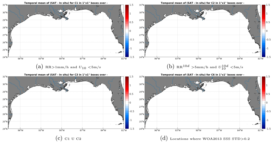
Figure 11: Temporal mean gridded over spatial boxes of size 1^\circ \times 1^\circ of \Delta SSS (SMOS-L4-CATDS-CECOS-IFREMER-V2-WEEKLY-0.5DEG - Surface drifters) for 4 different subdatasets corresponding to:RR >1 mm/h and U_{10} < 5 m/s (a), RR ^{10d} > 5 mm/h and U_{10}^{10d} < 5 m/s (b), C1 U C2 (c),Locations where WOA2013 SSS STD >0.2 (d).
