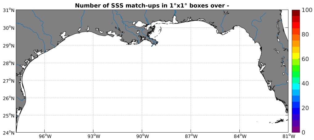
Figure 3: Number of SSS match-ups between Surface drifters SSS and the SMOS-L4-CATDS-CECOS-IFREMER-V2-WEEKLY-0.5DEG SSS product for the Mississippi river plume Pi-MEP region over 1^\circ \times 1^\circ boxes and for the full satellite product period.
