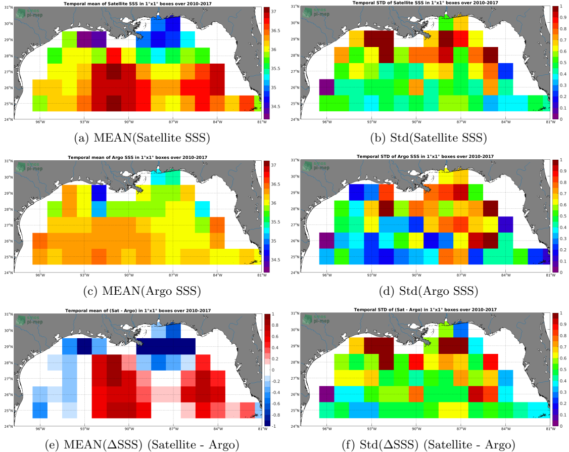
Figure 6: Temporal mean (left) and Std (right) of SSS from SMOS L4 v2 Weekly (CATDS-CECOS-IFREMER) (top), Argo (middle), and of \Delta\text{SSS} (Satellite - Argo). Only match-up pairs are used to generate these maps.
