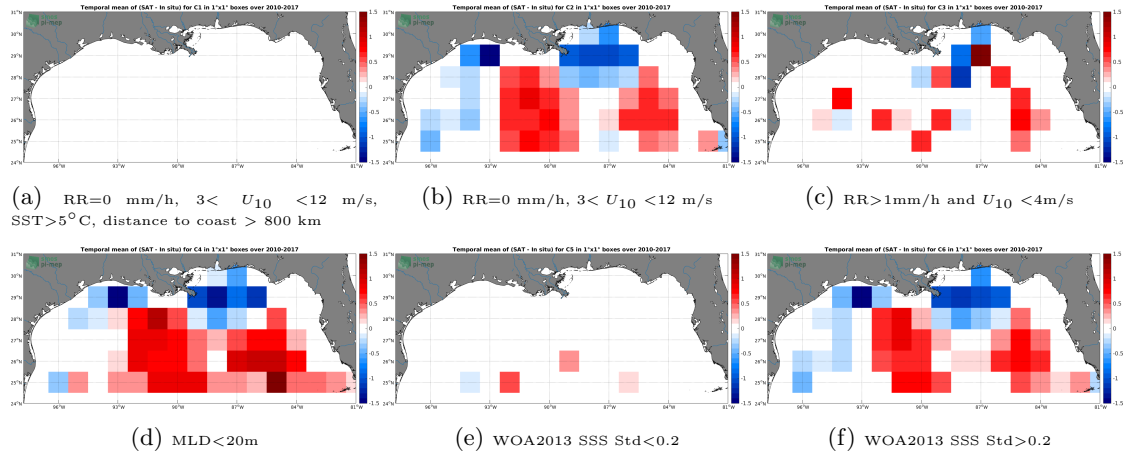
Figure 12: Temporal mean gridded over spatial boxes of size 1^{\circ}\times 1^{\circ} of \Delta\text{SSS} (SMOS-L4-CATDS-CECOS-IFREMER-V2-WEEKLY-0.5DEG - Argo) for 6 different subdatasets corresponding to: RR=0 mm/h, 3 < U_{10} < 12 m/s, SST > 5^{\circ}\text{C} , distance to coast > 800 km (a), RR=0 mm/h, 3 < U_{10} < 12 m/s (b), RR > 1\text{mm/h} and U_{10} < 4\text{m/s} (c), MLD < 20\text{m} (d), WOA2013 SSS Std < 0.2 (e), WOA2013 SSS Std > 0.2 (f).
