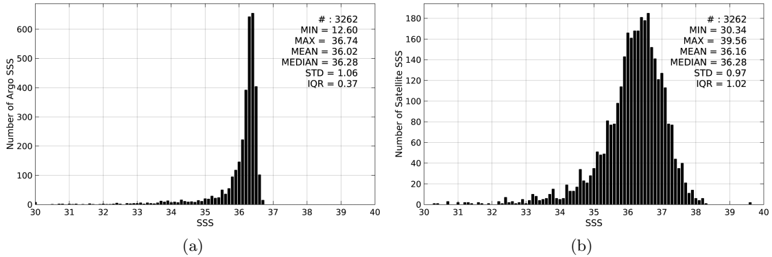
Figure 2: Histograms of SSS from Argo (a) and SMOS-L4-CATDS-CECOS-IFREMER-V2-WEEKLY-0.5DEG (b) considering all match-up pairs per bins of 0.1 over the Mississippi river plume Pi-MEP region and for the full satellite product period.
