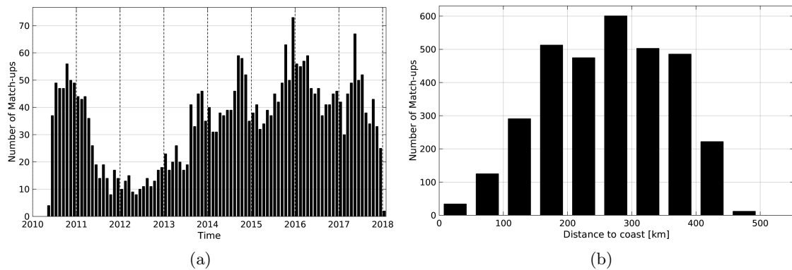
Figure 1: Number of match-ups between Argo and SMOS-L4-CATDS-CECOS-IFREMER-V2-WEEKLY-0.5DEG SSS as a function of time (a) and as function of the distance to coast (b) over the Mississippi river plume Pi-MEP region and for the full satellite product period.
