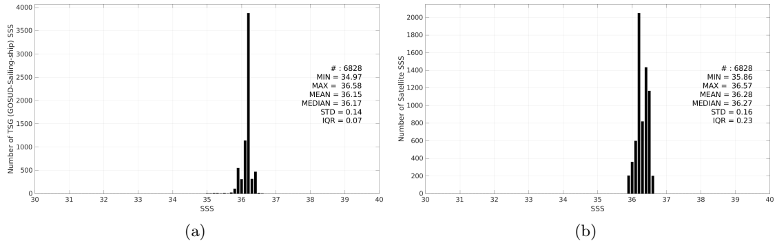
Figure 3: Histograms of SSS from TSG (GOSUD-Sailing-ship) (a) and SMOS SSS L4 v2 - Daily (BEC) (b) considering all match-up pairs per bins of 0.1 over the Mississippi river plume Pi-MEP region and for the full satellite product period.
