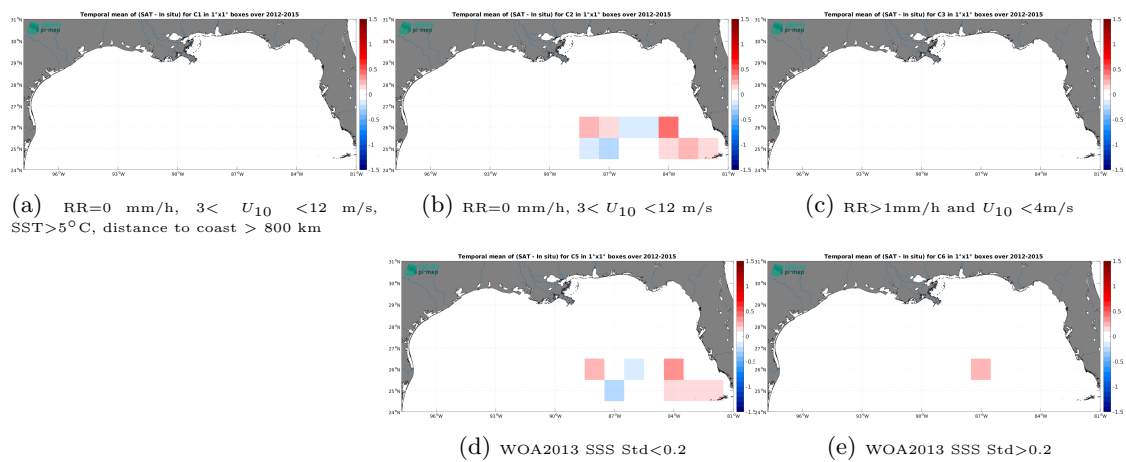
Figure 14: Temporal mean gridded over spatial boxes of size 1^\circ \times 1^\circ of \Delta SSS (SMOS SSS L4 v2 - Daily (BEC) - TSG (GOSUD-Sailing-ship)) for 5 different subdatasets corresponding to: RR=0 mm/h, 3 < U_{10} < 12 m/s, SST > 5°C, distance to coast > 800 km (a), RR=0 mm/h, 3 < U_{10} < 12 m/s (b), RR > 1mm/h and U_{10} < 4 m/s (c), WOA2013 SSS Std < 0.2 (d), WOA2013 SSS Std > 0.2 (e).
