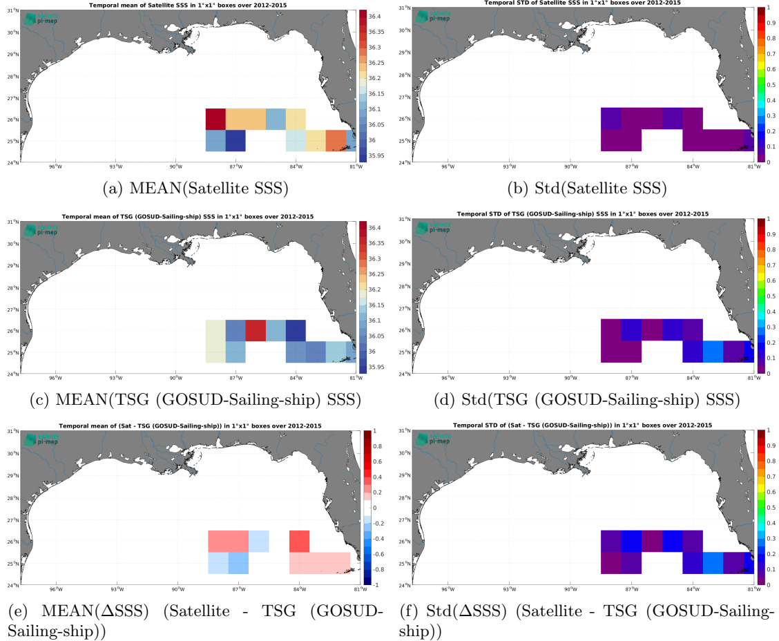
Figure 7: Temporal mean (left) and Std (right) of SSS from SMOS SSS L4 v2 - Daily (BEC) (top), TSG (GOSUD-Sailing-ship) (middle), and of \Delta\text{SSS} (Satellite - TSG (GOSUD-Sailing-ship)). Only match-up pairs are used to generate these maps.
