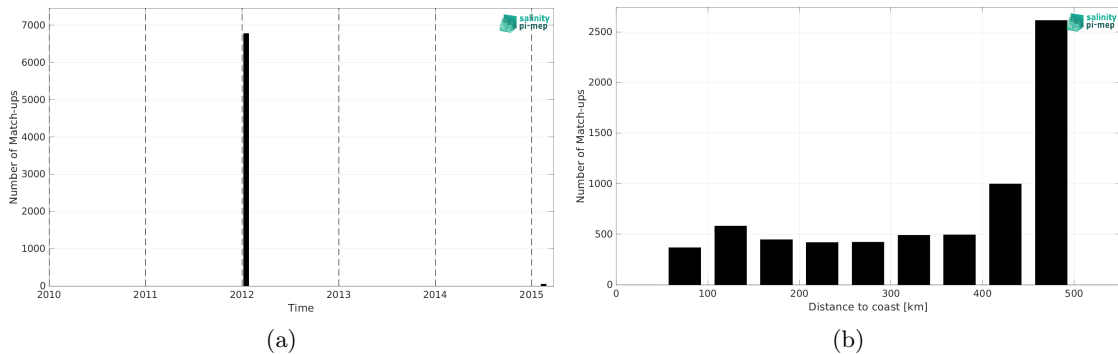
Figure 2: Number of match-ups between TSG (GOSUD-Sailing-ship) and SMOS SSS L4 v2 - Daily (BEC) SSS as a function of time (a) and as function of the distance to coast (b) over the Mississippi river plume Pi-MEP region and for the full satellite product period.
