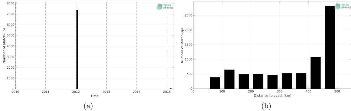
Figure 1: Number of match-ups between TSG (GOSUD-Sailing-ship) and SMOS SSS L4 v2 - Daily (BEC) SSS as a function of time (a) and as function of the distance to coast (b) over the Mississippi river plume Pi-MEP region and for the full satellite product period.
