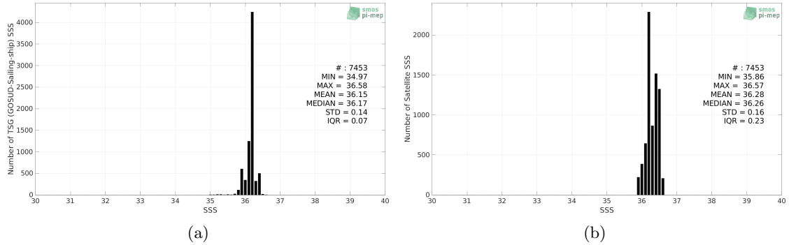
Figure 2: Histograms of SSS from TSG (GOSUD-Sailing-ship) (a) and SMOS SSS L4 v2 - Daily (BEC) (b) considering all match-up pairs per bins of 0.1 over the Mississippi river plume Pi-MEP region and for the full satellite product period.
