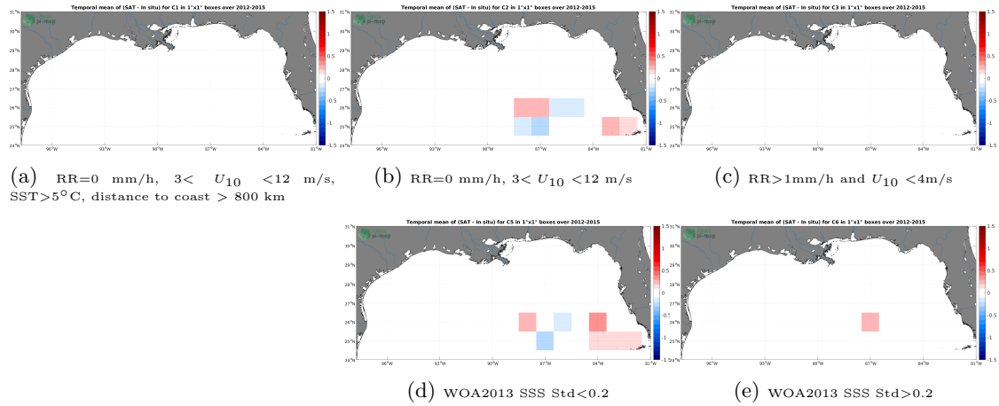
Figure 12: Temporal mean gridded over spatial boxes of size 1^{\circ}\times 1^{\circ} of \Delta SSS (SMOS SSS L4 v2 - Daily (BEC) - TSG (GOSUD-Sailing-ship)) for 5 different subdatasets corresponding to:RR=0 mm/h, 3 < U_{10} < 12 m/s, SST >5^{\circ}\text{C} , distance to coast > 800 km (a), RR=0 mm/h, 3 < U_{10} < 12 m/s (b), RR >1 mm/h and U_{10} < 4 m/s (c), WOA2013 SSS Std <0.2 (d), WOA2013 SSS Std >0.2 (e).
