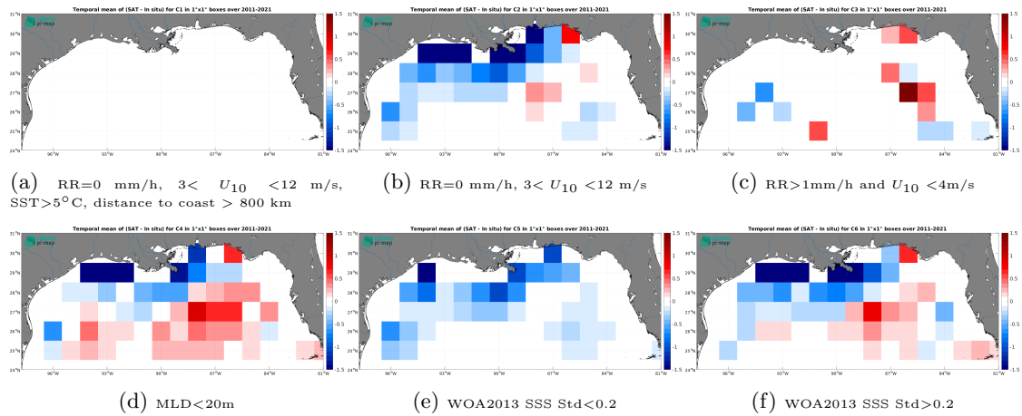
Figure 14: Temporal mean gridded over spatial boxes of size 1^\circ \times 1^\circ of \Delta SSS (SMOS SSS L4 v2 - Daily (BEC) - Argo) for 6 different subdatasets corresponding to:RR=0 mm/h, 3 < U_{10} < 12 m/s, SST > 5^\circ\text{C} , distance to coast > 800 km (a), RR=0 mm/h, 3 < U_{10} < 12 m/s (b), RR > 1 mm/h and U_{10} < 4 m/s (c),MLD < 20 m (d),WOA2013 SSS Std < 0.2 (e),WOA2013 SSS Std > 0.2 (f).
