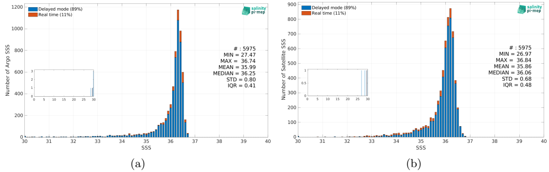
Figure 3: Histograms of SSS from Argo (a) and SMOS SSS L4 v2 - Daily (BEC) (b) considering all match-up pairs per bins of 0.1 over the Mississippi river plume Pi-MEP region and for the full satellite product period.
