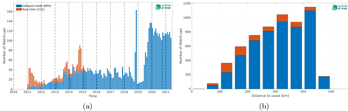
Figure 2: Number of match-ups between Argo and SMOS SSS L4 v2 - Daily (BEC) SSS as a function of time (a) and as function of the distance to coast (b) over the Mississippi river plume Pi-MEP region and for the full satellite product period.
