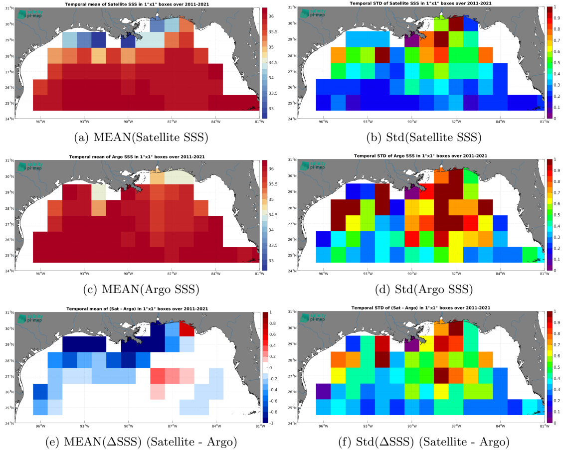
Figure 7: Temporal mean (left) and Std (right) of SSS from SMOS SSS L4 v2 - Daily (BEC) (top), Argo (middle), and of \Delta\text{SSS} (Satellite - Argo). Only match-up pairs are used to generate these maps.
