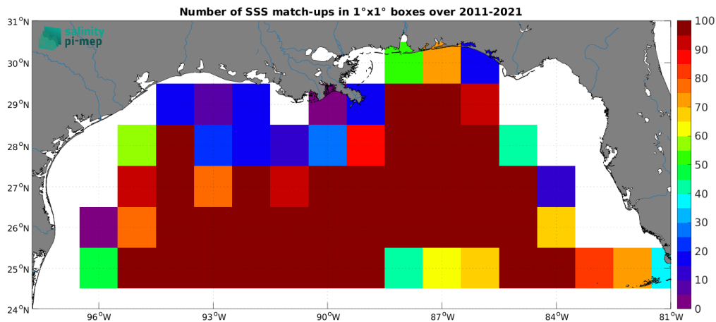
Figure 5: Number of SSS match-ups between Argo SSS and the SMOS SSS L4 v2 - Daily (BEC) SSS product for the Mississippi river plume Pi-MEP region over 1^\circ \times 1^\circ boxes and for the full satellite product period.
