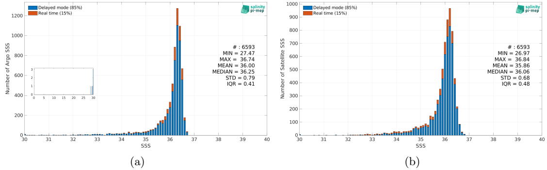
Figure 2: Histograms of SSS from Argo (a) and SMOS SSS L4 v2 - Daily (BEC) (b) considering all match-up pairs per bins of 0.1 over the Mississippi river plume Pi-MEP region and for the full satellite product period.
