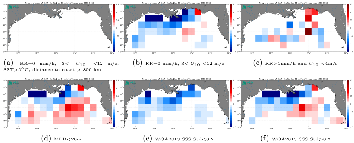
Figure 12: Temporal mean gridded over spatial boxes of size 1^{\circ}\times 1^{\circ} of \Delta\text{SSS} (SMOS SSS L4 v2 - Daily (BEC) - Argo) for 6 different subdatasets corresponding to:RR=0 mm/h, 3 < U_{10} < 12 m/s, SST > 5^{\circ}\text{C} , distance to coast > 800 km (a), RR=0 mm/h, 3 < U_{10} < 12 m/s (b), RR > 1\text{mm/h} and U_{10} < 4\text{m/s} (c),MLD < 20\text{m} (d),WOA2013 SSS Std < 0.2 (e),WOA2013 SSS Std > 0.2 (f).
