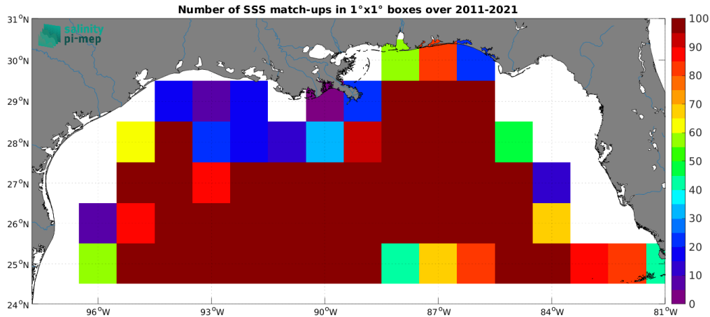
Figure 4: Number of SSS match-ups between Argo SSS and the SMOS SSS L4 v2 - Daily (BEC) SSS product for the Mississippi river plume Pi-MEP region over 1^\circ \times 1^\circ boxes and for the full satellite product period.
