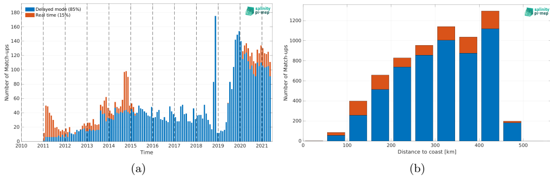
Figure 1: Number of match-ups between Argo and SMOS SSS L4 v2 - Daily (BEC) SSS as a function of time (a) and as function of the distance to coast (b) over the Mississippi river plume Pi-MEP region and for the full satellite product period.
