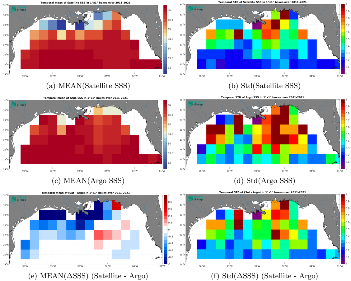
Figure 6: Temporal mean (left) and Std (right) of SSS from SMOS SSS L4 v2 - Daily (BEC) (top), Argo (middle), and of \Delta\text{SSS} (Satellite - Argo). Only match-up pairs are used to generate these maps.
