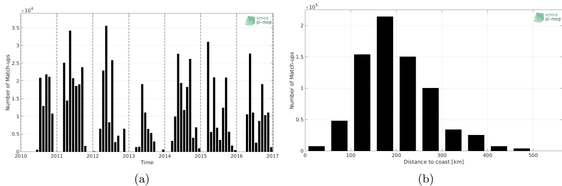
Figure 1: Number of match-ups between TSG-SAMOS and SMOS-L3-ICDC-V3-MONTHLY-0.5DEG SSS as a function of time (a) and as function of the distance to coast (b) over the Mississippi river plume Pi-MEP region and for the full satellite product period.
