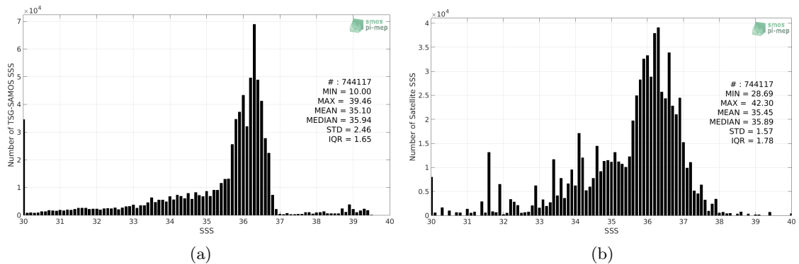
Figure 2: Histograms of SSS from TSG-SAMOS (a) and SMOS-L3-ICDC-V3-MONTHLY-0.5DEG (b) considering all match-up pairs per bins of 0.1 over the Mississippi river plume Pi-MEP region and for the full satellite product period.
