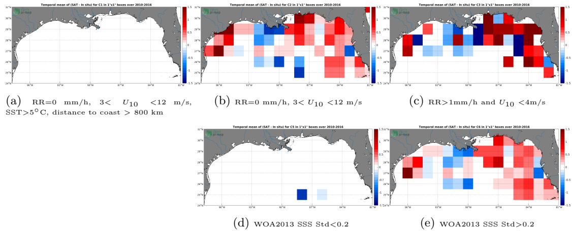
Figure 12: Temporal mean gridded over spatial boxes of size 1^\circ \times 1^\circ of \Delta SSS (SMOS-L3-ICDC-V3-MONTHLY-0.5DEG - TSG-SAMOS) for 5 different subdatasets corresponding to:RR=0 mm/h, 3 < U_{10} < 12 m/s, SST >5^\circ\text{C} , distance to coast > 800 km (a), RR=0 mm/h, 3 < U_{10} < 12 m/s (b), RR >1 mm/h and U_{10} < 4 m/s (c), WOA2013 SSS Std <0.2 (d), WOA2013 SSS Std >0.2 (e).
