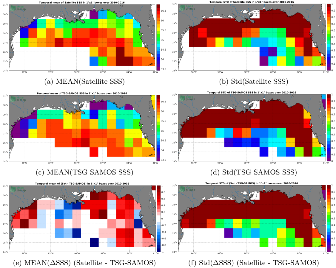
Figure 6: Temporal mean (left) and Std (right) of SSS from SMOS-L3-ICDC-V3-MONTHLY-0.5DEG (top), TSG-SAMOS (middle), and of \Delta SSS (Satellite - TSG-SAMOS). Only match-up pairs are used to generate these maps.
