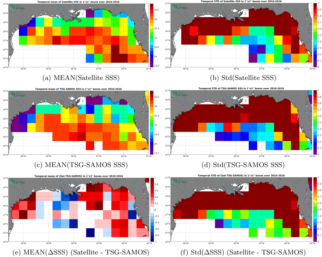
Figure 6: Temporal mean (left) and Std (right) of SSS from SMOS-L3-ICDC-V3-MONTHLY-0.5DEG (top), TSG-SAMOS (middle), and of \Delta\text{SSS} (Satellite - TSG-SAMOS). Only match-up pairs are used to generate these maps.
