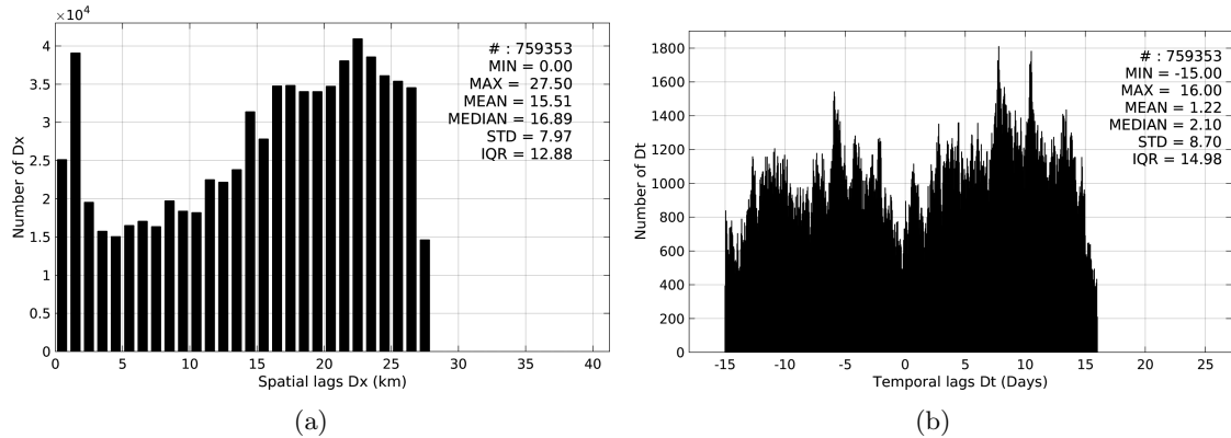
Figure 5: Histograms of the spatial (a) and temporal (b) lags between the time of the TSG-SAMOS measurements and the date of the corresponding SMOS-L3-ICDC-V3-MONTHLY-0.5DEG SSS product.
