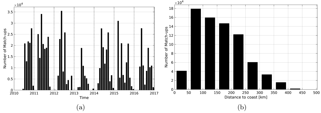
Figure 1: Number of match-ups between TSG-SAMOS and SMOS-L3-ICDC-V3-MONTHLY-0.5DEG SSS as a function of time (a) and as function of the distance to coast (b) over the Mississippi river plume Pi-MEP region and for the full satellite product period.
