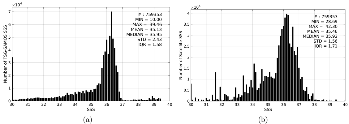
Figure 2: Histograms of SSS from TSG-SAMOS (a) and SMOS-L3-ICDC-V3-MONTHLY-0.5DEG (b) considering all match-up pairs per bins of 0.1 over the Mississippi river plume Pi-MEP region and for the full satellite product period.
