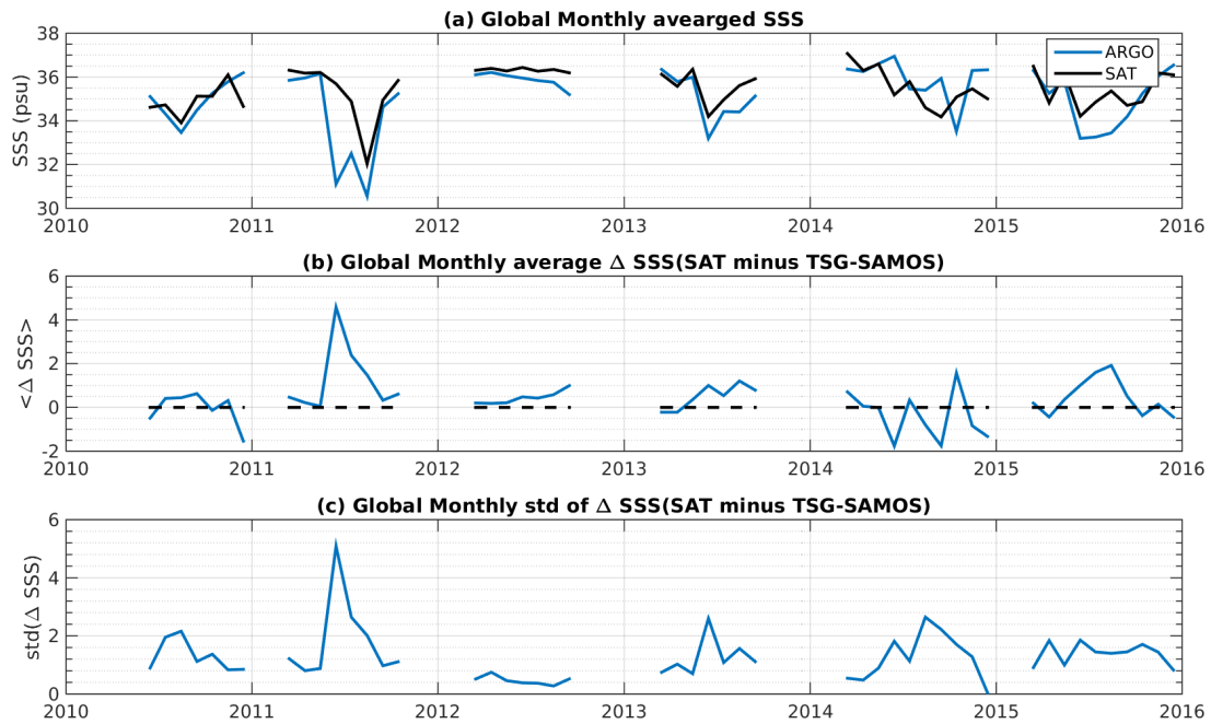
Figure 7: Time series of the monthly averaged mean SSS (top), mean \Delta SSS (Satellite - TSG-SAMOS) and STD of \Delta SSS (Satellite - TSG-SAMOS) over the Mississippi river plume Pi-MEP region considering all match-ups collected by the Pi-MEP platform.
