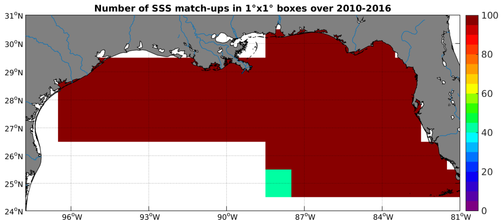
Figure 4: Number of SSS match-ups between TSG-SAMOS SSS and the SMOS-L3-ICDC-V3-MONTHLY-0.5DEG SSS product for the Mississippi river plume Pi-MEP region over 1^\circ \times 1^\circ boxes and for the full satellite product period.
