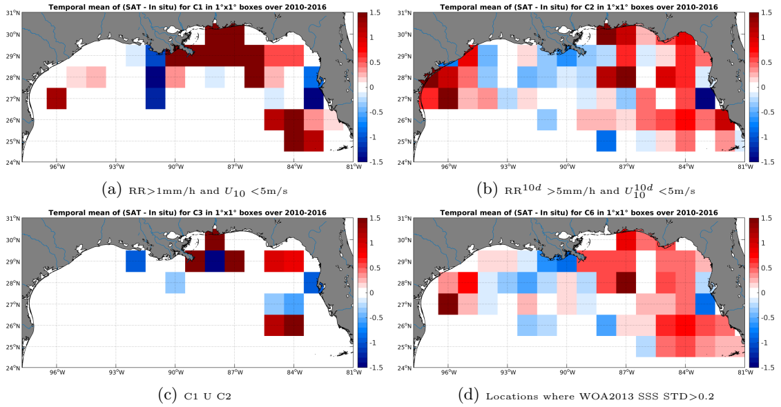
Figure 12: Temporal mean gridded over spatial boxes of size 1^\circ \times 1^\circ of \Delta SSS (SMOS-L3-ICDC-V3-MONTHLY-0.5DEG - TSG-SAMOS) for 4 different subdatasets corresponding to: RR > 1 mm/h and U_{10} < 5 m/s (a), RR 10d > 5 mm/h and U_{10}^{10d} < 5 m/s (b), C1 U C2 (c), Locations where WOA2013 SSS STD > 0.2 (d).
