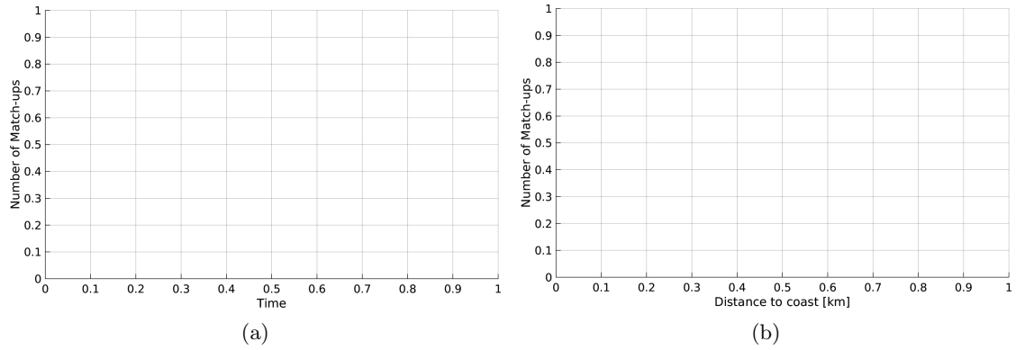
Figure 1: Number of match-ups between TSG-LEGOS-DM and SMOS-L3-ICDC-V3-MONTHLY-0.5DEG SSS as a function of time (a) and as function of the distance to coast (b) over the Mississippi river plume Pi-MEP region and for the full satellite product period.
