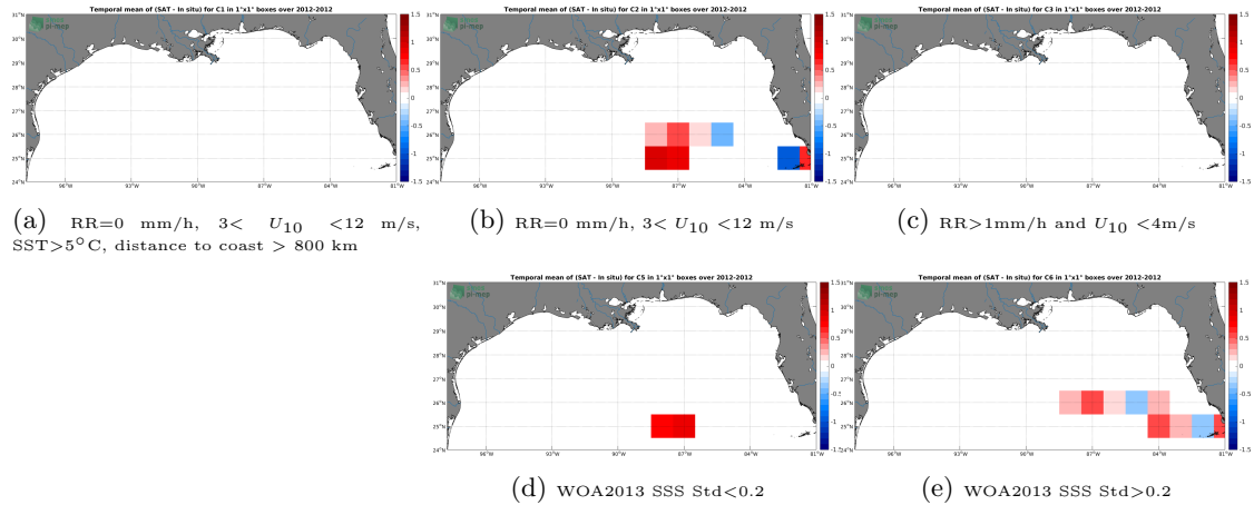
Figure 12: Temporal mean gridded over spatial boxes of size 1^{\circ}\times 1^{\circ} of \Delta SSS (SMOS SSS L3 v3 Monthly (ICDC) - TSG (GOSUD-Sailing-ship)) for 5 different subdatasets corresponding to: RR=0 mm/h, 3 < U_{10} < 12 m/s, SST > 5^{\circ}\text{C} , distance to coast > 800 km (a), RR=0 mm/h, 3 < U_{10} < 12 m/s (b), RR > 1 mm/h and U_{10} < 4 m/s (c), WOA2013 SSS Std < 0.2 (d), WOA2013 SSS Std > 0.2 (e).
