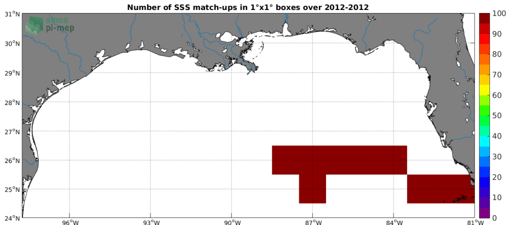
Figure 4: Number of SSS match-ups between TSG (GOSUD-Sailing-ship) SSS and the SMOS SSS L3 v3 Monthly (ICDC) SSS product for the Mississippi river plume Pi-MEP region over 1°x1° boxes and for the full satellite product period.
