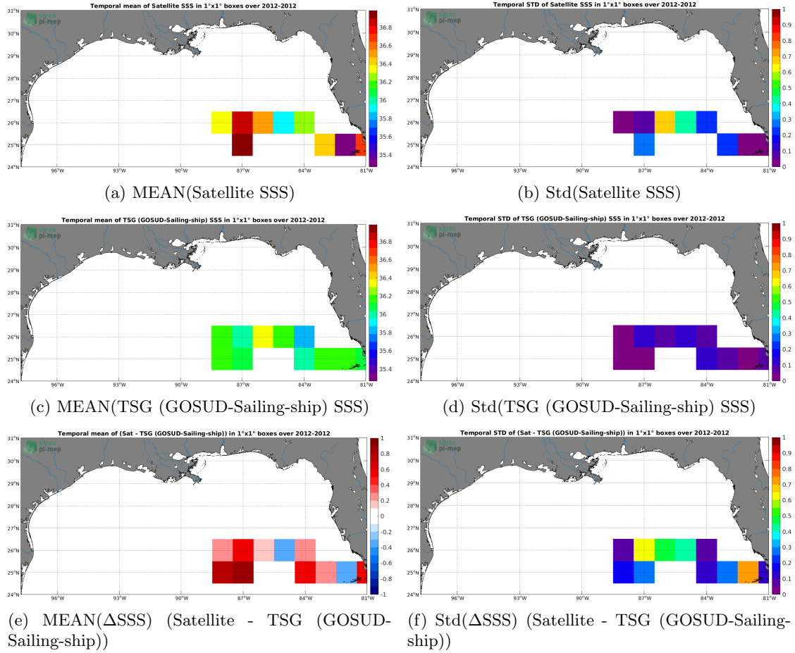
Figure 6: Temporal mean (left) and Std (right) of SSS from SMOS SSS L3 v3 Monthly (ICDC) (top), TSG (GOSUD-Sailing-ship) (middle), and of \Delta SSS (Satellite - TSG (GOSUD-Sailing-ship)). Only match-up pairs are used to generate these maps.
