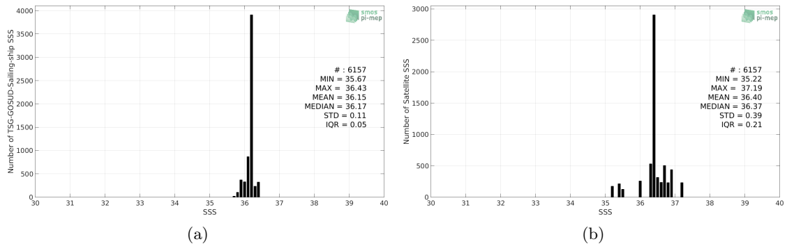
Figure 2: Histograms of SSS from TSG-GOSUD-Sailing-ship (a) and SMOS-L3-ICDC-V3-MONTHLY-0.5DEG (b) considering all match-up pairs per bins of 0.1 over the Mississippi river plume Pi-MEP region and for the full satellite product period.
