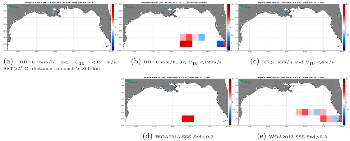
Figure 12: Temporal mean gridded over spatial boxes of size 1^{\circ}\times 1^{\circ} of \Delta SSS (SMOS-L3-ICDC-V3-MONTHLY-0.5DEG - TSG-GOSUD-Sailing-ship) for 5 different subdatasets corresponding to:RR=0 mm/h, 3 < U_{10} < 12 m/s, SST >5^{\circ}\text{C} , distance to coast > 800 km (a), RR=0 mm/h, 3 < U_{10} < 12 m/s (b), RR >1 mm/h and U_{10} < 4 m/s (c), WOA2013 SSS Std <0.2 (d), WOA2013 SSS Std >0.2 (e).
