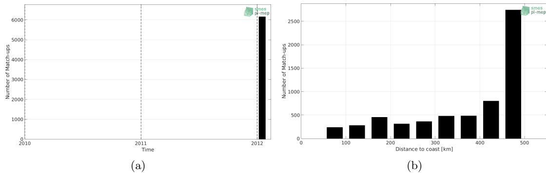
Figure 1: Number of match-ups between TSG-GOSUD-Sailing-ship and SMOS-L3-ICDC-V3-MONTHLY-0.5DEG SSS as a function of time (a) and as function of the distance to coast (b) over the Mississippi river plume Pi-MEP region and for the full satellite product period.
