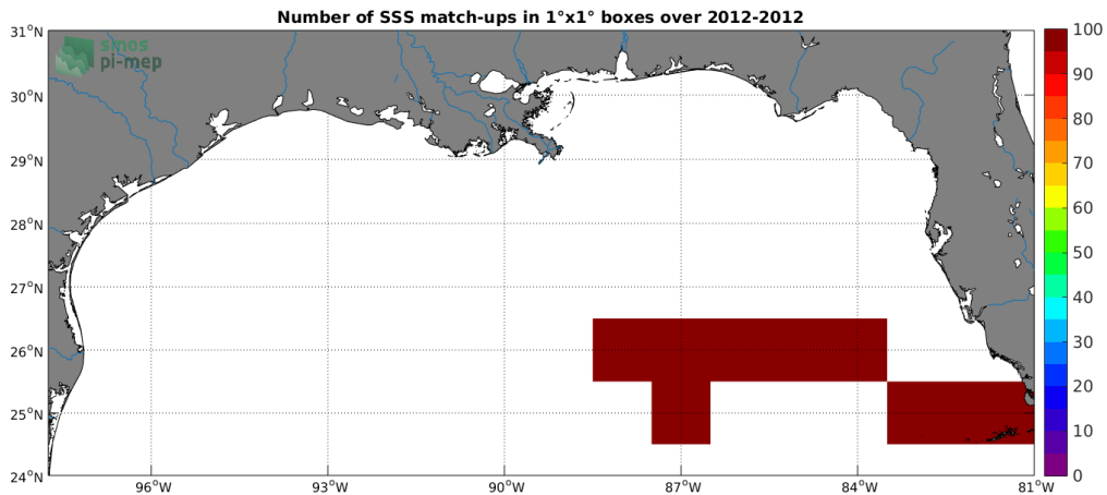
Figure 4: Number of SSS match-ups between TSG-GOSUD-Sailing-ship SSS and the SMOS-L3-ICDC-V3-MONTHLY-0.5DEG SSS product for the Mississippi river plume Pi-MEP region over 1^\circ \times 1^\circ boxes and for the full satellite product period.
