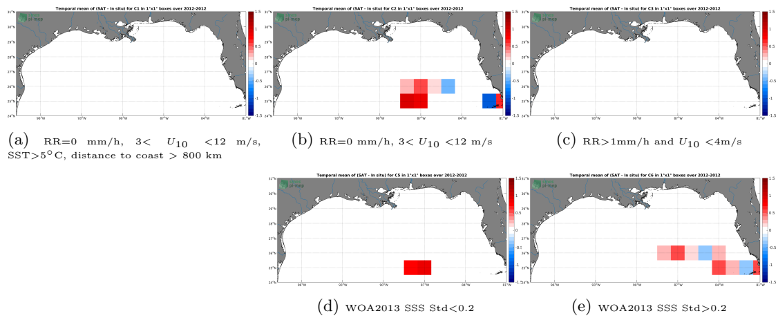
Figure 12: Temporal mean gridded over spatial boxes of size 1^\circ \times 1^\circ of \Delta SSS (SMOS-L3-ICDC-V3-MONTHLY-0.5DEG - TSG-GOSUD-Sailing-ship) for 5 different subdatasets corresponding to:RR=0 mm/h, 3 < U_{10} < 12 m/s, SST >5^\circ C, distance to coast > 800 km (a), RR=0 mm/h, 3 < U_{10} < 12 m/s (b), RR >1 mm/h and U_{10} < 4 m/s (c), WOA2013 SSS Std <0.2 (d), WOA2013 SSS Std >0.2 (e).
