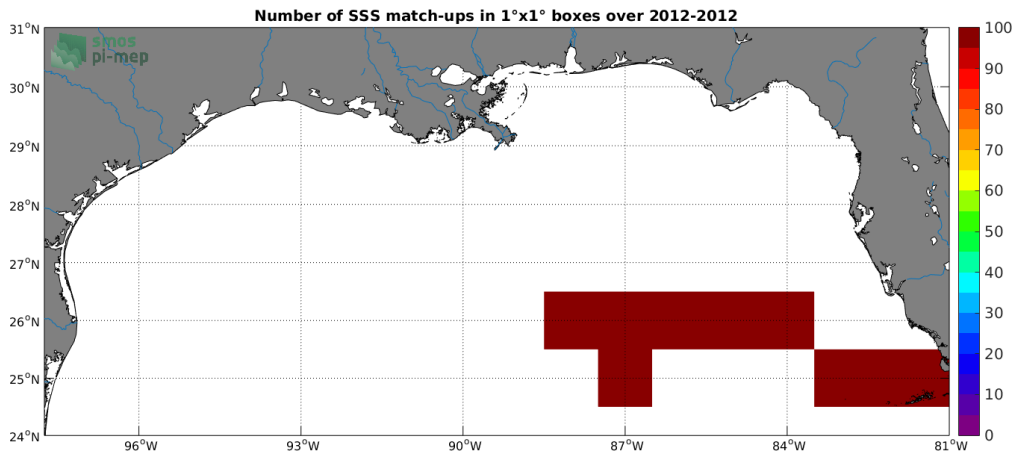
Figure 4: Number of SSS match-ups between TSG-GOSUD-Sailing-ship SSS and the SMOS-L3-ICDC-V3-MONTHLY-0.5DEG SSS product for the Mississippi river plume Pi-MEP region over 1°x1° boxes and for the full satellite product period.
