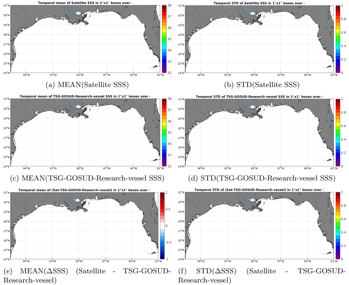
Figure 6: Temporal mean (left) and STD (right) of SSS from SMOS-L3-ICDC-V3-MONTHLY-0.5DEG (top), TSG-GOSUD-Research-vessel (middle), and of \Delta SSS (Satellite - TSG-GOSUD-Research-vessel). Only match-up pairs are used to generate these maps.
