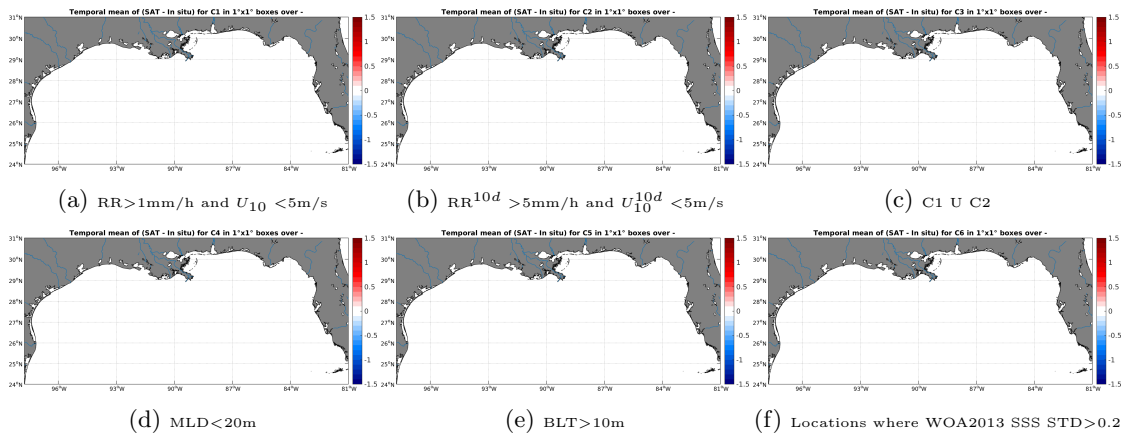
Figure 12: Temporal mean gridded over spatial boxes of size 1^\circ \times 1^\circ of \Delta SSS (SMOS-L3-ICDC-V3-MONTHLY-0.5DEG - Sea mammals) for 6 different subdatasets corresponding to:RR >1 mm/h and U_{10} < 5 m/s (a), RR ^{10d} > 5 mm/h and U_{10}^{10d} < 5 m/s (b), C1 U C2 (c),MLD <20 m (d),BLT >10 m (e),Locations where WOA2013 SSS STD >0.2 (f).
