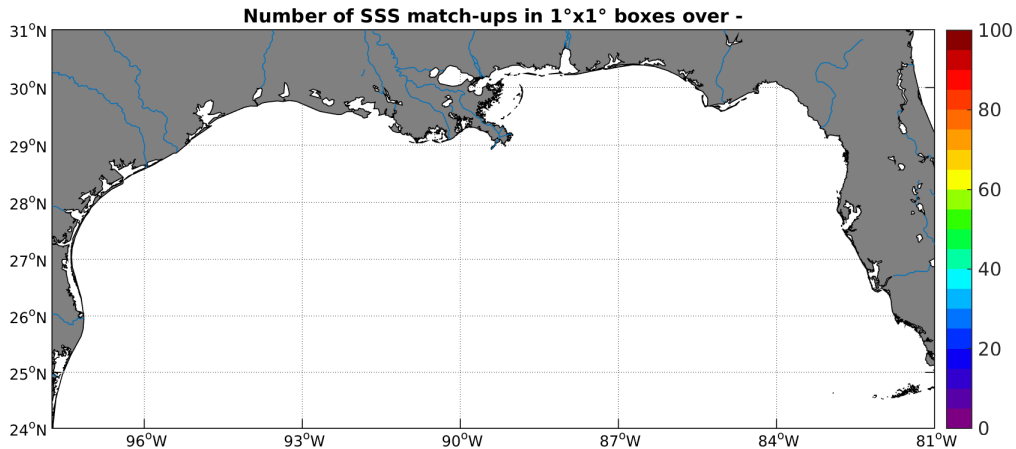
Figure 3: Number of SSS match-ups between Surface drifters SSS and the SMOS-L3-ICDC-V3-MONTHLY-0.5DEG SSS product for the Mississippi river plume Pi-MEP region over 1^\circ \times 1^\circ boxes and for the full satellite product period.
