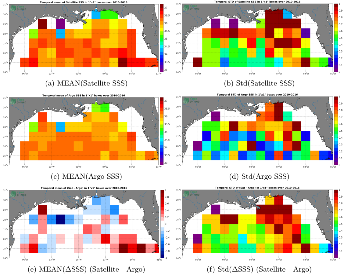
Figure 6: Temporal mean (left) and Std (right) of SSS from SMOS SSS L3 v3 Monthly (ICDC) (top), Argo (middle), and of \Delta\text{SSS} (Satellite - Argo). Only match-up pairs are used to generate these maps.
