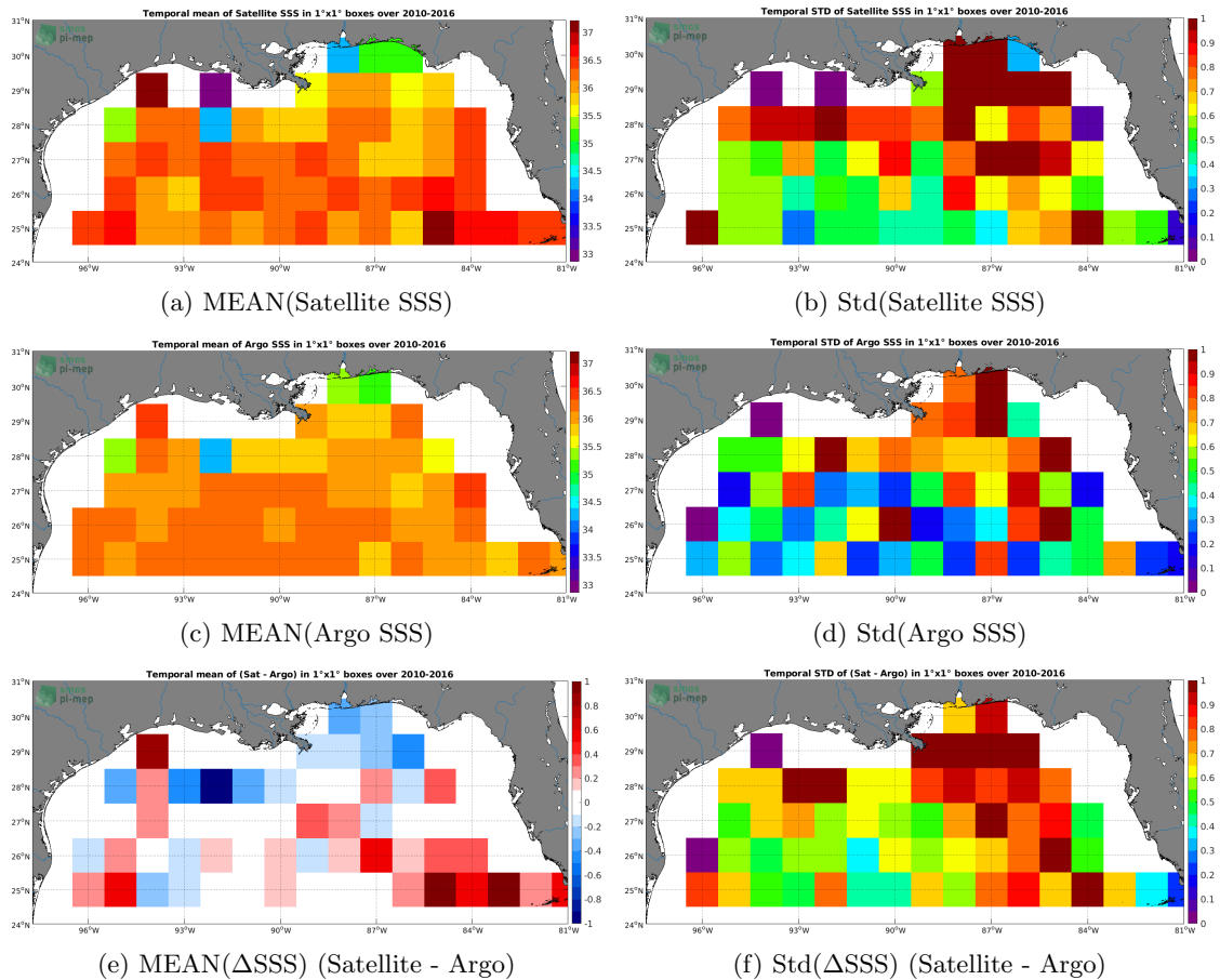
Figure 6: Temporal mean (left) and Std (right) of SSS from SMOS SSS L3 v3 Monthly (ICDC) (top), Argo (middle), and of \Delta\text{SSS} (Satellite - Argo). Only match-up pairs are used to generate these maps.
