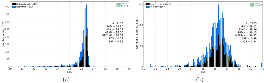
Figure 2: Histograms of SSS from Argo (a) and SMOS SSS L3 v3 Monthly (ICDC) (b) considering all match-up pairs per bins of 0.1 over the Mississippi river plume Pi-MEP region and for the full satellite product period.
