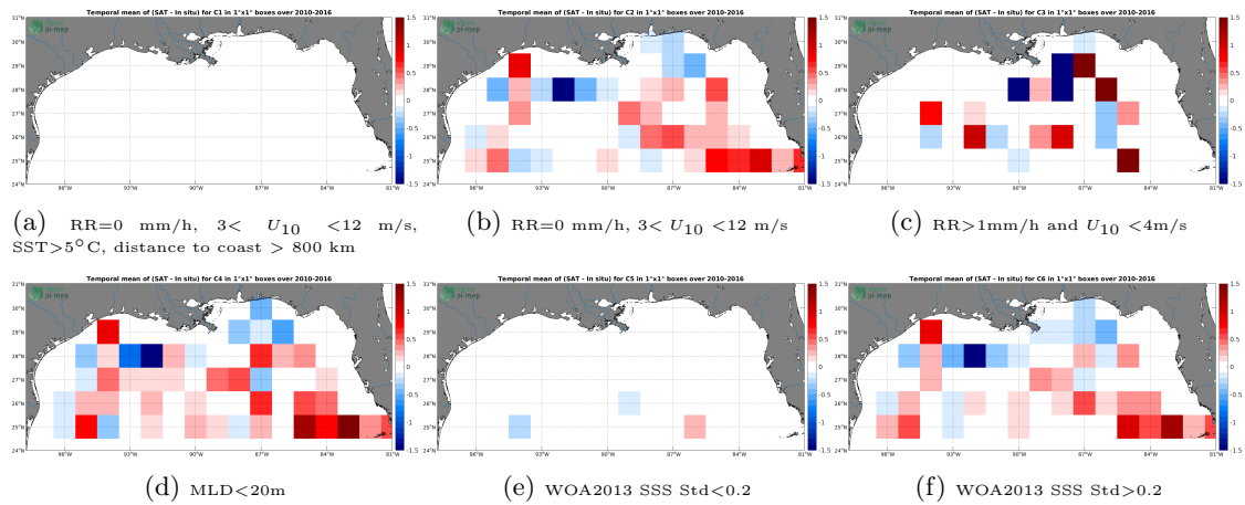
Figure 12: Temporal mean gridded over spatial boxes of size 1^{\circ}\times 1^{\circ} of \Delta\text{SSS} (SMOS SSS L3 v3 Monthly (ICDC) - Argo) for 6 different subdatasets corresponding to:RR=0 mm/h, 3 < U_{10} < 12 m/s, SST > 5^{\circ}\text{C} , distance to coast > 800 km (a), RR=0 mm/h, 3 < U_{10} < 12 m/s (b), RR > 1\text{mm/h} and U_{10} < 4\text{m/s} (c),MLD < 20\text{m} (d),WOA2013 SSS Std < 0.2 (e),WOA2013 SSS Std > 0.2 (f).
