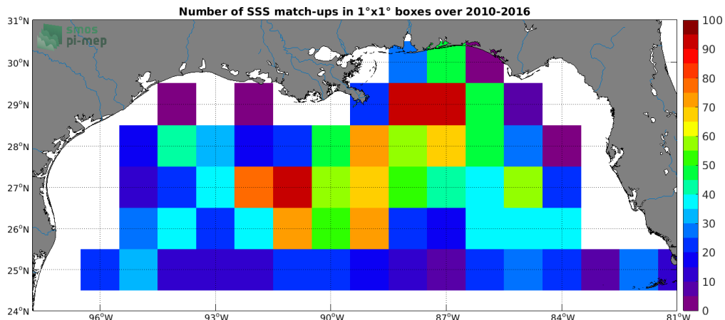
Figure 4: Number of SSS match-ups between Argo SSS and the SMOS SSS L3 v3 Monthly (ICDC) SSS product for the Mississippi river plume Pi-MEP region over 1^\circ \times 1^\circ boxes and for the full satellite product period.
