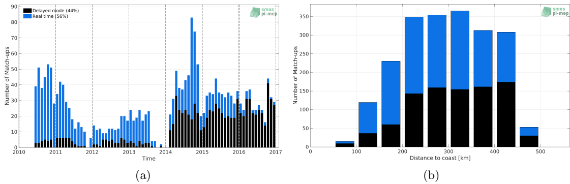
Figure 1: Number of match-ups between Argo and SMOS SSS L3 v3 Monthly (ICDC) SSS as a function of time (a) and as function of the distance to coast (b) over the Mississippi river plume Pi-MEP region and for the full satellite product period.
