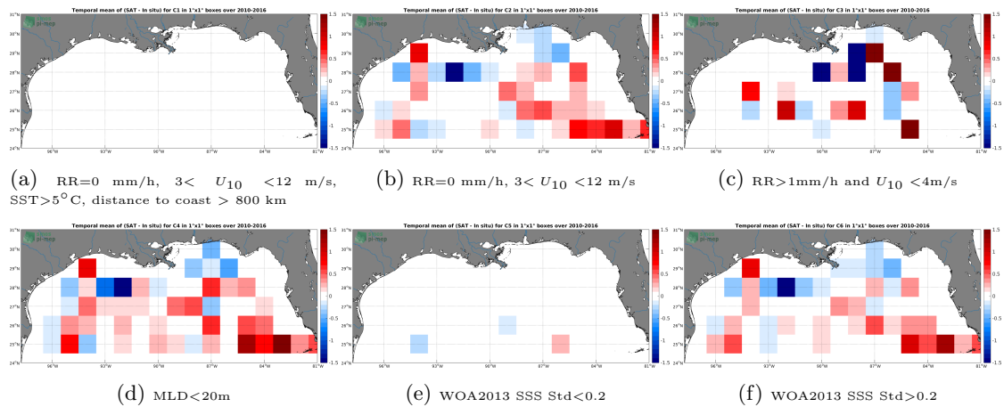
Figure 12: Temporal mean gridded over spatial boxes of size 1^{\circ}\times 1^{\circ} of \Delta\text{SSS} (SMOS-L3-ICDC-V3-MONTHLY-0.5DEG - Argo) for 6 different subdatasets corresponding to:RR=0 mm/h, 3 < U_{10} < 12 m/s, SST > 5^{\circ}\text{C} , distance to coast > 800 km (a), RR=0 mm/h, 3 < U_{10} < 12 m/s (b), RR > 1 mm/h and U_{10} < 4 m/s (c),MLD < 20\text{m} (d),WOA2013 SSS Std < 0.2 (e),WOA2013 SSS Std > 0.2 (f).
