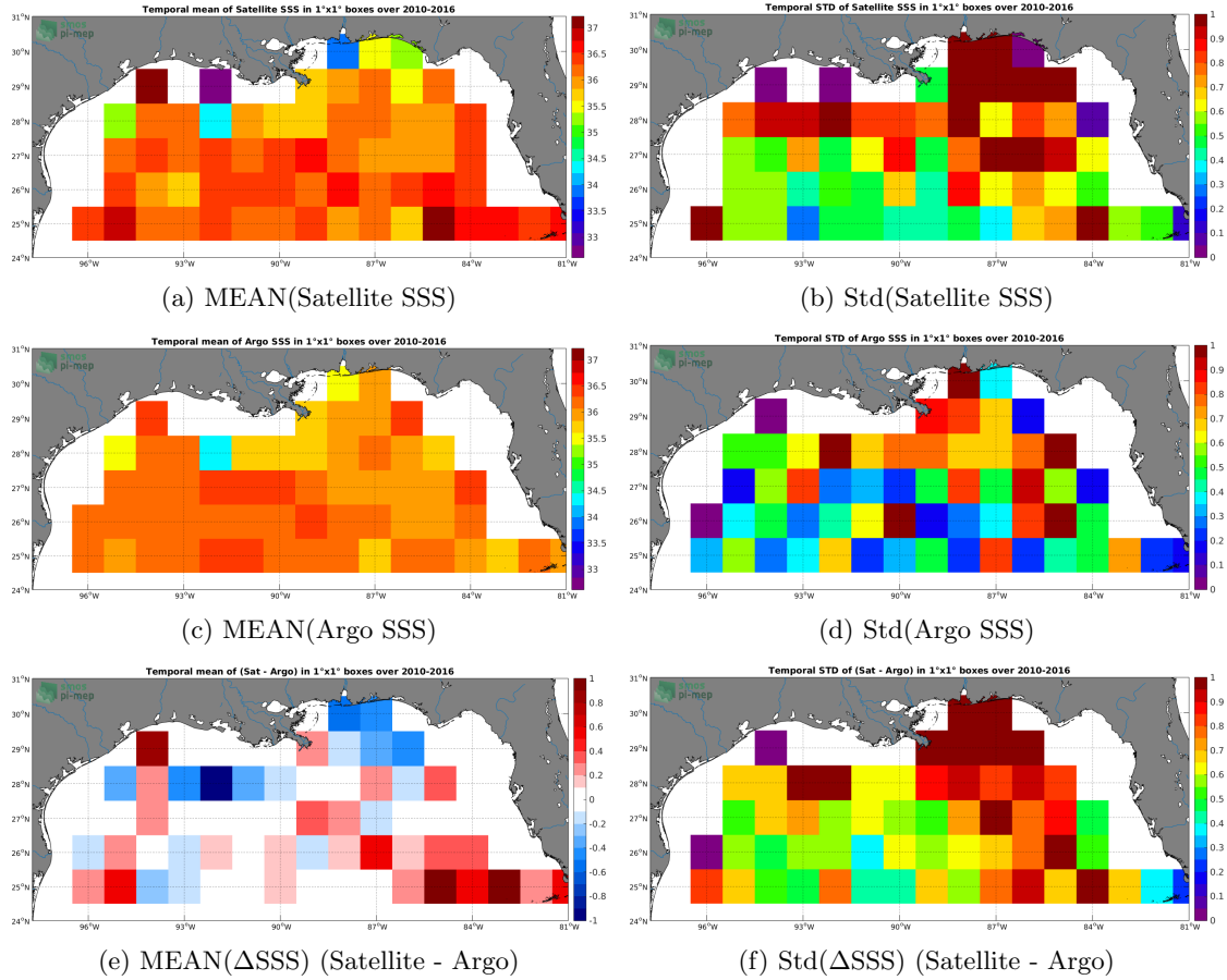
Figure 6: Temporal mean (left) and Std (right) of SSS from SMOS-L3-ICDC-V3-MONTHLY-0.5DEG (top), Argo (middle), and of \Delta SSS (Satellite - Argo). Only match-up pairs are used to generate these maps.
