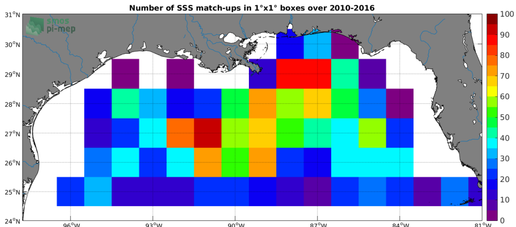
Figure 4: Number of SSS match-ups between Argo SSS and the SMOS-L3-ICDC-V3-MONTHLY-0.5DEG SSS product for the Mississippi river plume Pi-MEP region over 1°x1° boxes and for the full satellite product period.
