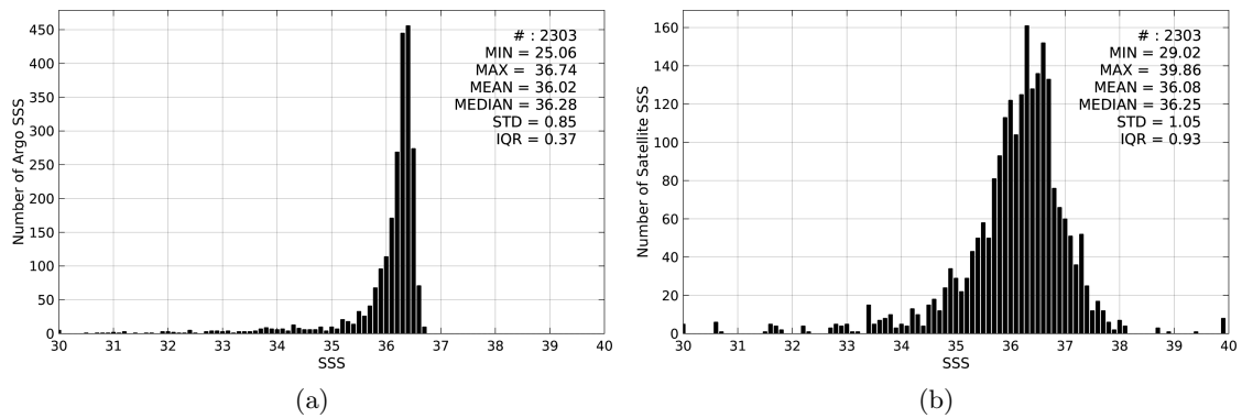
Figure 2: Histograms of SSS from Argo (a) and SMOS-L3-ICDC-V3-MONTHLY-0.5DEG (b) considering all match-up pairs per bins of 0.1 over the Mississippi river plume Pi-MEP region and for the full satellite product period.
