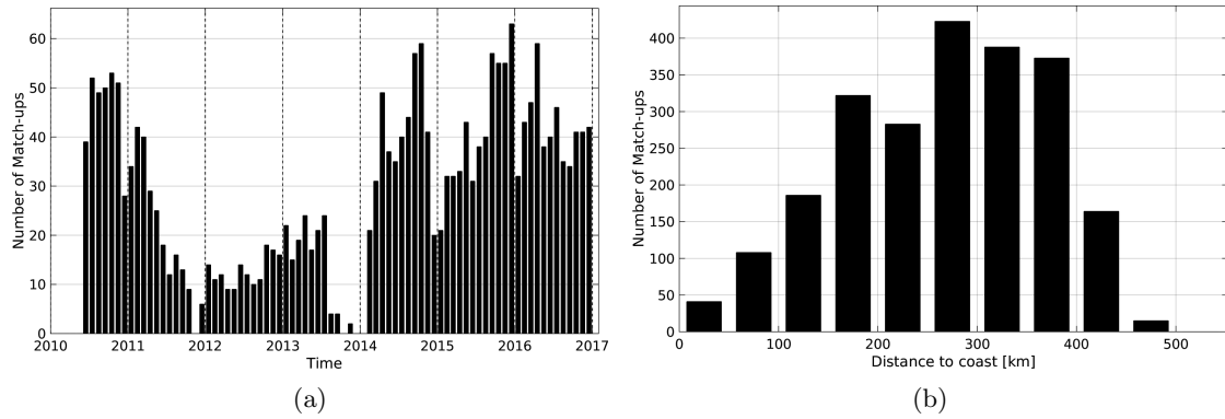
Figure 1: Number of match-ups between Argo and SMOS-L3-ICDC-V3-MONTHLY-0.5DEG SSS as a function of time (a) and as function of the distance to coast (b) over the Mississippi river plume Pi-MEP region and for the full satellite product period.
