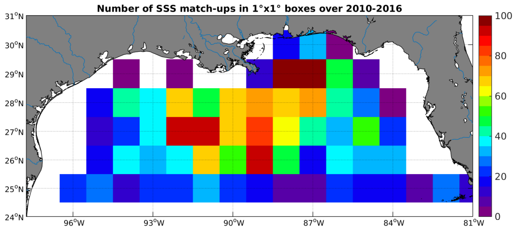
Figure 4: Number of SSS match-ups between Argo SSS and the SMOS-L3-ICDC-V3-MONTHLY-0.5DEG SSS product for the Mississippi river plume Pi-MEP region over 1^{\circ} \times 1^{\circ} boxes and for the full satellite product period.
