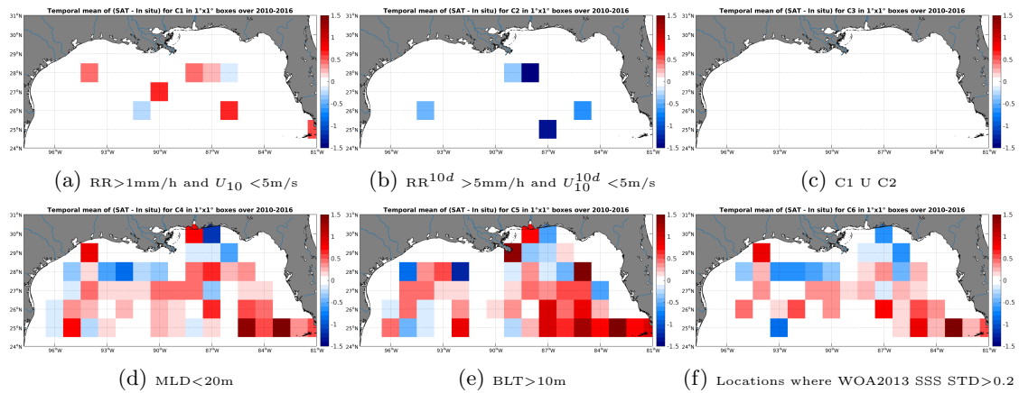
Figure 12: Temporal mean gridded over spatial boxes of size 1^\circ \times 1^\circ of \Delta SSS (SMOS-L3-ICDC-V3-MONTHLY-0.5DEG - Argo) for 6 different subdatasets corresponding to: RR > 1\text{mm/h} and U_{10} < 5\text{m/s} (a), RR^{10d} > 5\text{mm/h} and U_{10}^{10d} < 5\text{m/s} (b), C1 U C2 (c), MLD < 20\text{m} (d), BLT > 10\text{m} (e), Locations where WOA2013 SSS STD > 0.2 (f).
