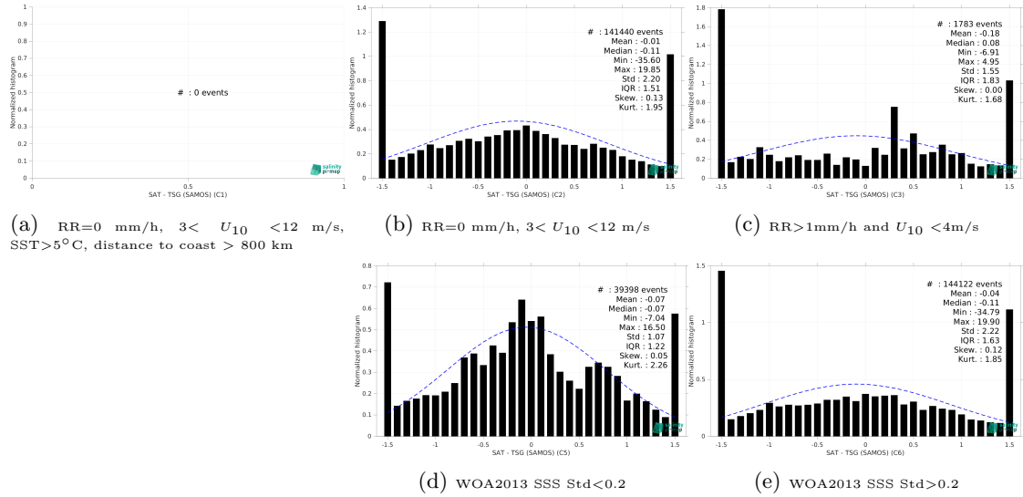
Figure 15: Normalized histogram of \Delta SSS (SMOS SSS L2Q v331 - With FLAG (CMEMS-CATDS-CPDC) - TSG (SAMOS)) for 5 different subdatasets corresponding to: RR=0 mm/h, 3 < U_{10} < 12 m/s, SST > 5°C, distance to coast > 800 km (a), RR=0 mm/h, 3 < U_{10} < 12 m/s (b), RR > 1mm/h and U_{10} < 4 m/s (c), WOA2013 SSS Std < 0.2 (d), WOA2013 SSS Std > 0.2 (e).
