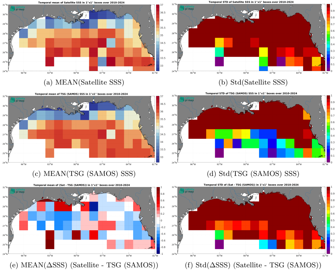
Figure 7: Temporal mean (left) and Std (right) of SSS from SMOS SSS L2Q v331 - With FLAG (CMEMS-CATDS-CPDC) (top), TSG (SAMOS) (middle), and of \Delta\text{SSS} (Satellite - TSG (SAMOS)). Only match-up pairs are used to generate these maps.
