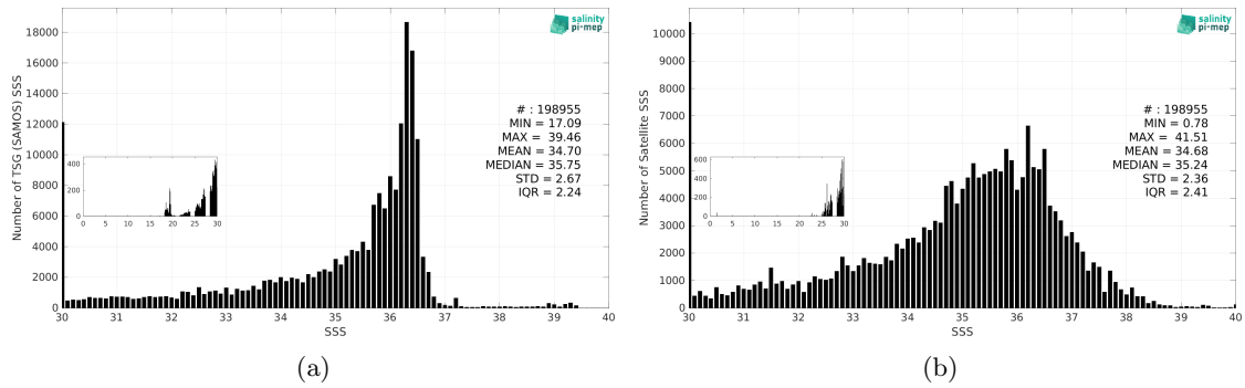
Figure 3: Histograms of SSS from TSG (SAMOS) (a) and SMOS SSS L2Q v331 - With FLAG (CMEMS-CATDS-CPDC) (b) considering all match-up pairs per bins of 0.1 over the Mississippi river plume Pi-MEP region and for the full satellite product period.
