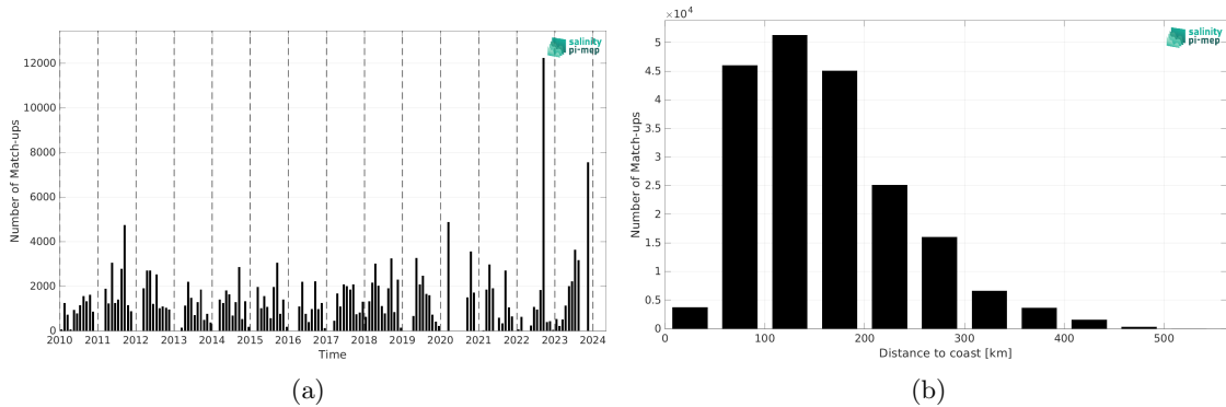
Figure 2: Number of match-ups between TSG (SAMOS) and SMOS SSS L2Q v331 - With FLAG (CMEMS-CATDS-CPDC) SSS as a function of time (a) and as function of the distance to coast (b) over the Mississippi river plume Pi-MEP region and for the full satellite product period.
