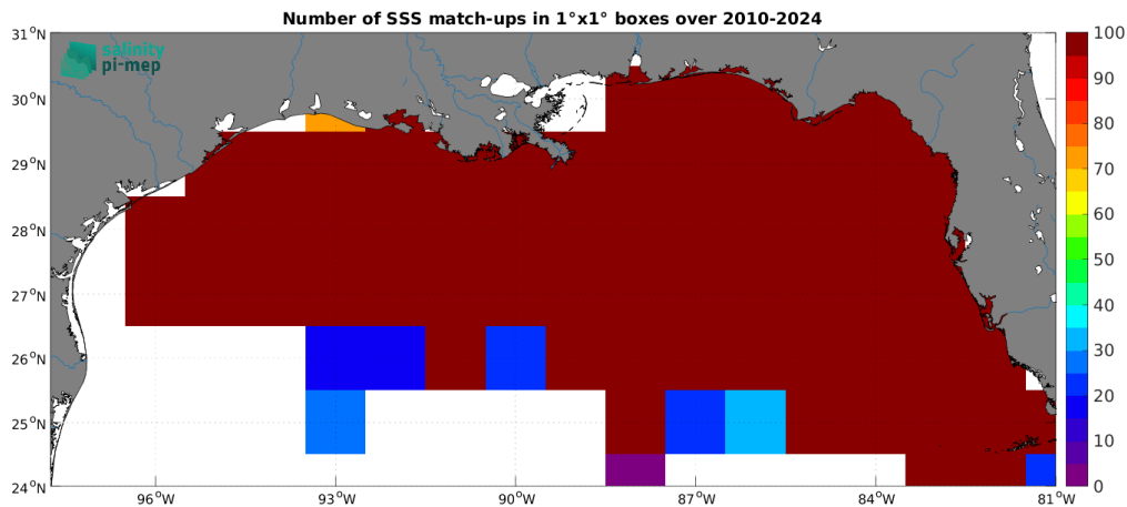
Figure 5: Number of SSS match-ups between TSG (SAMOS) SSS and the SMOS SSS L2Q v331 - With FLAG (CMEMS-CATDS-CPDC) SSS product for the Mississippi river plume Pi-MEP region over 1^\circ \times 1^\circ boxes and for the full satellite product period.
