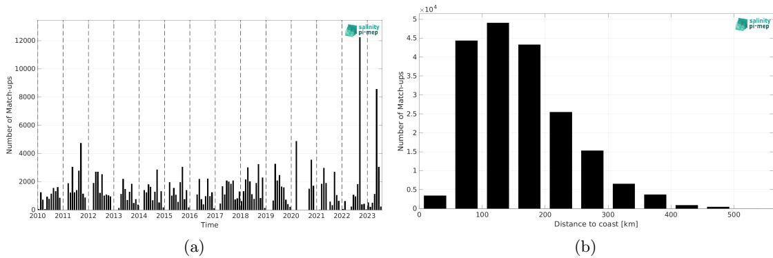
Figure 1: Number of match-ups between TSG (SAMOS) and SMOS SSS L2Q v331 - With FLAG (CMEMS-CATDS-CPDC) SSS as a function of time (a) and as function of the distance to coast (b) over the Mississippi river plume Pi-MEP region and for the full satellite product period.
