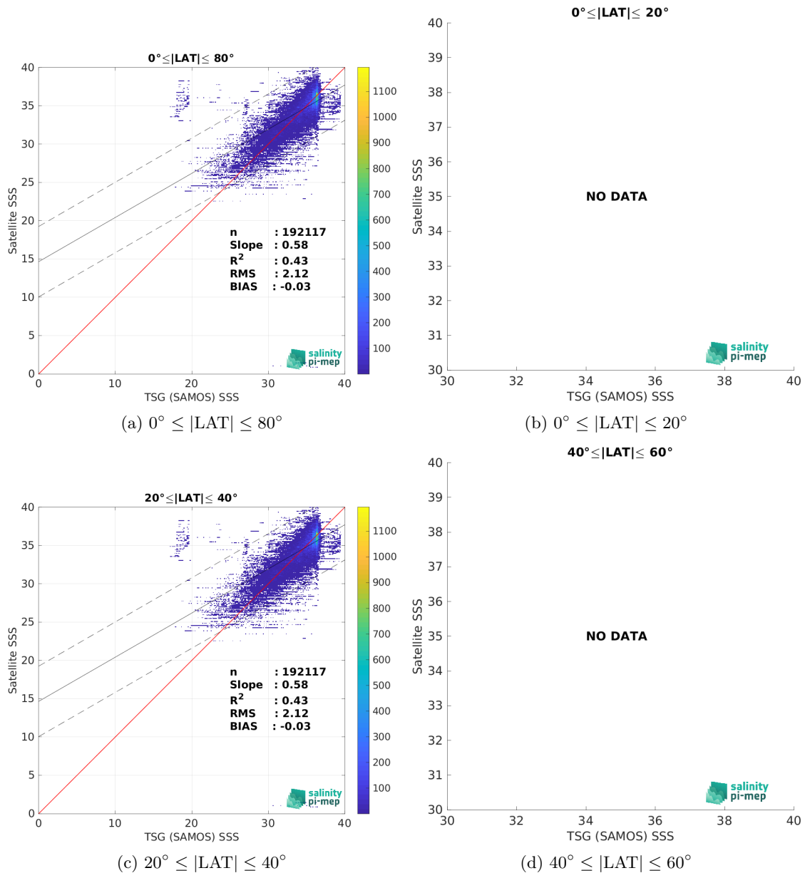
Figure 9: Contour maps of the concentration of SMOS SSS L2Q v331 - With FLAG (CMEMS-CATDS-CPDC) SSS (y-axis) versus TSG (SAMOS) SSS (x-axis) at match-up pairs for different latitude bands. For each plot, the red line shows x=y . The black thin and dashed lines indicate a linear fit through the data cloud and the \pm 95\% confidence levels, respectively. The number match-up pairs n , the slope and R^2 coefficient of the linear fit, the root mean square (RMS) and the mean bias between satellite and in situ data are indicated for each latitude band in each plots.
