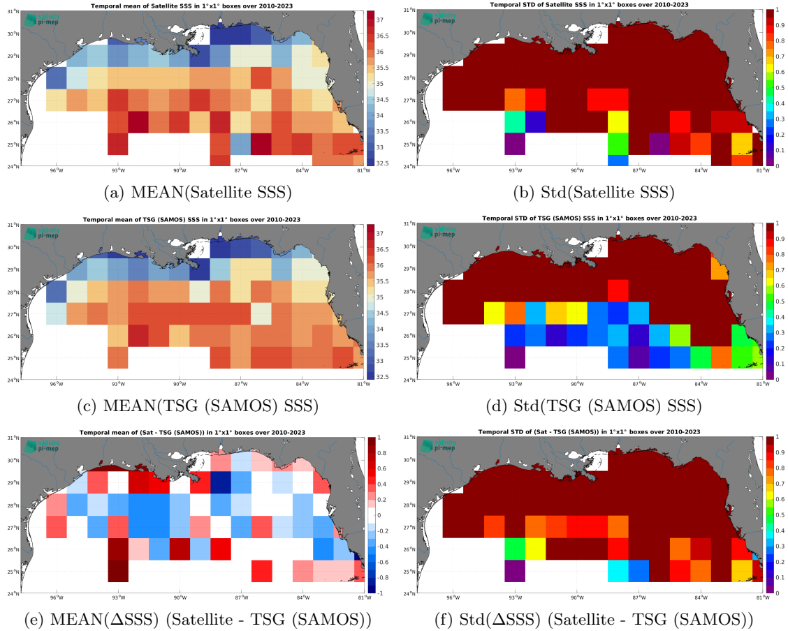
Figure 6: Temporal mean (left) and Std (right) of SSS from SMOS SSS L2Q v331 - With FLAG (CMEMS-CATDS-CPDC) (top), TSG (SAMOS) (middle), and of \Delta\text{SSS} (Satellite - TSG (SAMOS)). Only match-up pairs are used to generate these maps.
