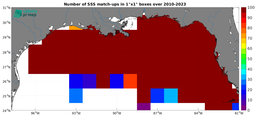
Figure 4: Number of SSS match-ups between TSG (SAMOS) SSS and the SMOS SSS L2Q v331 - With FLAG (CMEMS-CATDS-CPDC) SSS product for the Mississippi river plume Pi-MEP region over 1^\circ \times 1^\circ boxes and for the full satellite product period.
