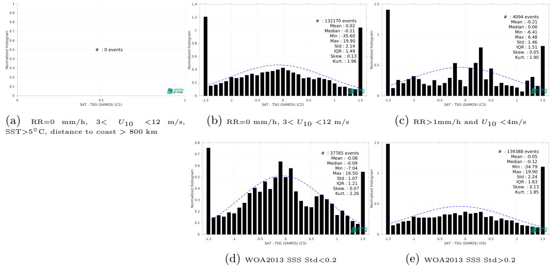
Figure 13: Normalized histogram of \Delta SSS (SMOS SSS L2Q v331 - With FLAG (CMEMS-CATDS-CPDC) - TSG (SAMOS)) for 5 different subdatasets corresponding to: RR=0 mm/h, 3 < U_{10} < 12 m/s, SST > 5°C, distance to coast > 800 km (a), RR=0 mm/h, 3 < U_{10} < 12 m/s (b), RR > 1mm/h and U_{10} < 4 m/s (c), WOA2013 SSS Std < 0.2 (d), WOA2013 SSS Std > 0.2 (e).
