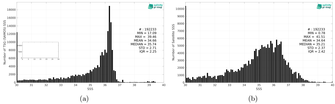
Figure 2: Histograms of SSS from TSG (SAMOS) (a) and SMOS SSS L2Q v331 - With FLAG (CMEMS-CATDS-CPDC) (b) considering all match-up pairs per bins of 0.1 over the Mississippi river plume Pi-MEP region and for the full satellite product period.
