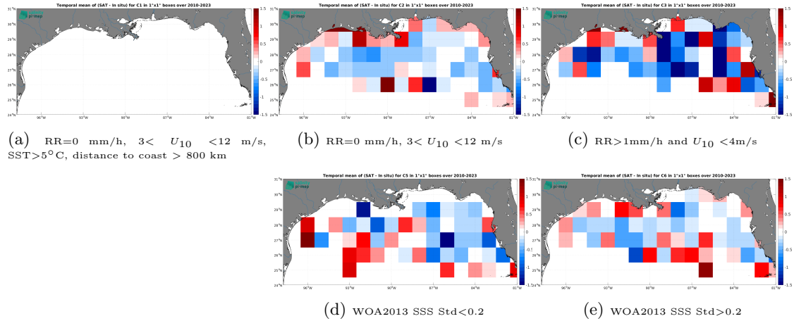
Figure 12: Temporal mean gridded over spatial boxes of size 1^{\circ}\times 1^{\circ} of \Delta\text{SSS} (SMOS SSS L2Q v331 - With FLAG (CMEMS-CATDS-CPDC) - TSG (SAMOS)) for 5 different subdatasets corresponding to:RR=0 mm/h, 3 < U_{10} < 12 m/s, SST >5^{\circ}\text{C} , distance to coast > 800 km (a), RR=0 mm/h, 3 < U_{10} < 12 m/s (b), RR >1 mm/h and U_{10} < 4 m/s (c), WOA2013 SSS Std <0.2 (d), WOA2013 SSS Std >0.2 (e).
