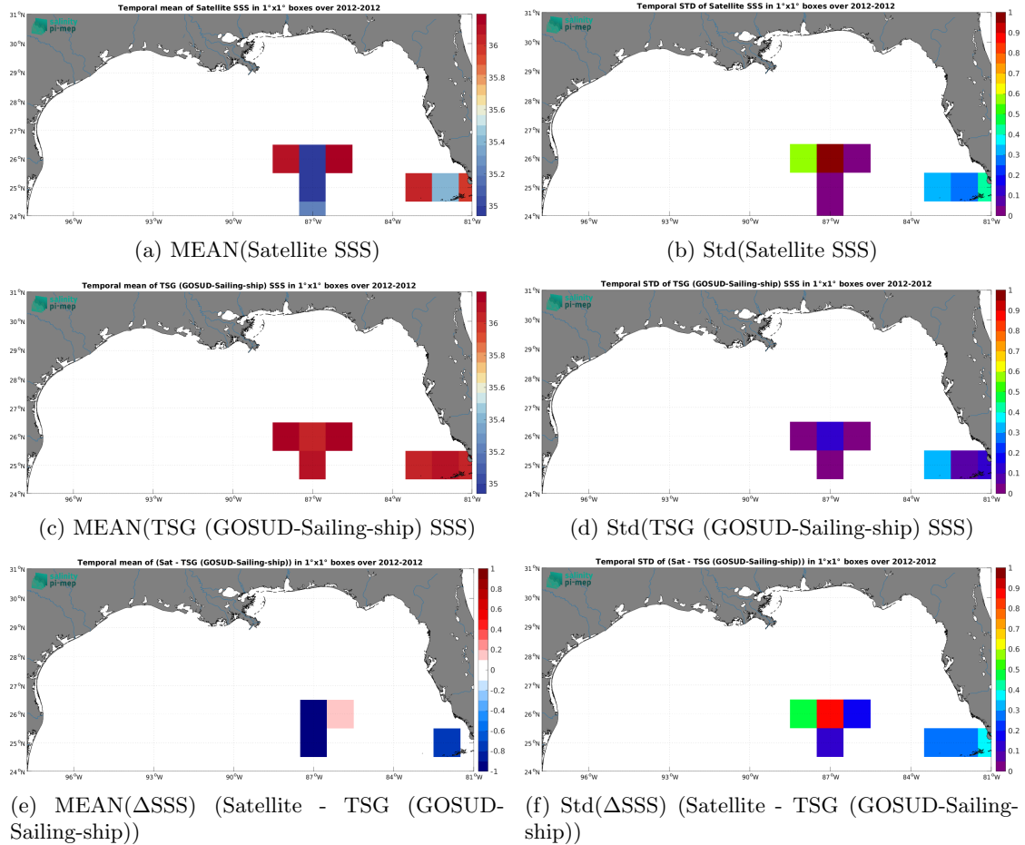
Figure 7: Temporal mean (left) and Std (right) of SSS from SMOS SSS L2Q v331 - With FLAG (CMEMS-CATDS-CPDC) (top), TSG (GOSUD-Sailing-ship) (middle), and of \Delta\text{SSS} (Satellite - TSG (GOSUD-Sailing-ship)). Only match-up pairs are used to generate these maps.
