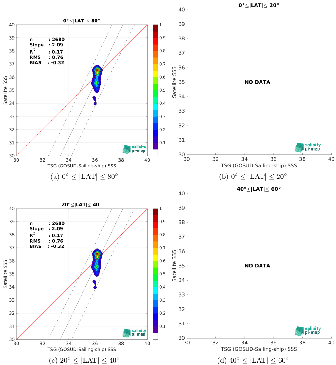
Figure 10: Contour maps of the concentration of SMOS SSS L2Q v331 - With FLAG (CMEMS-CATDS-CPDC) SSS (y-axis) versus TSG (GOSUD-Sailing-ship) SSS (x-axis) at match-up pairs for different latitude bands. For each plot, the red line shows x=y . The black thin and dashed lines indicate a linear fit through the data cloud and the \pm 95\% confidence levels, respectively. The number match-up pairs n , the slope and R^2 coefficient of the linear fit, the root mean square (RMS) and the mean bias between satellite and in situ data are indicated for each latitude band in each plots.
