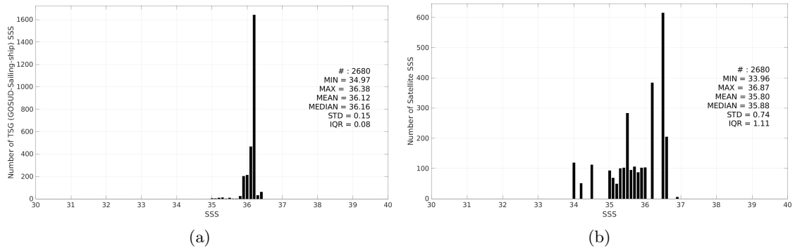
Figure 3: Histograms of SSS from TSG (GOSUD-Sailing-ship) (a) and SMOS SSS L2Q v331 - With FLAG (CMEMS-CATDS-CPDC) (b) considering all match-up pairs per bins of 0.1 over the Mississippi river plume Pi-MEP region and for the full satellite product period.
