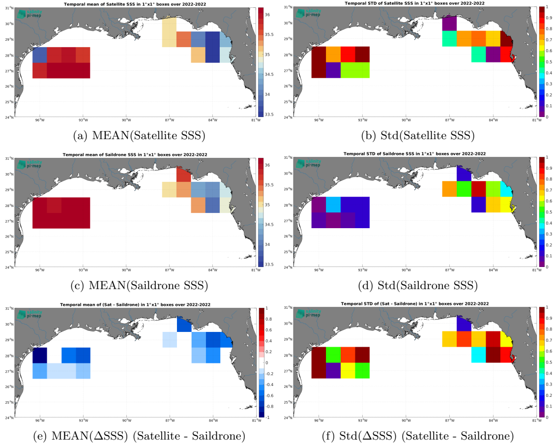
Figure 7: Temporal mean (left) and Std (right) of SSS from SMOS SSS L2Q v331 - With FLAG (CMEMS-CATDS-CPDC) (top), Sairdrone (middle), and of \Delta SSS (Satellite - Sairdrone). Only match-up pairs are used to generate these maps.
