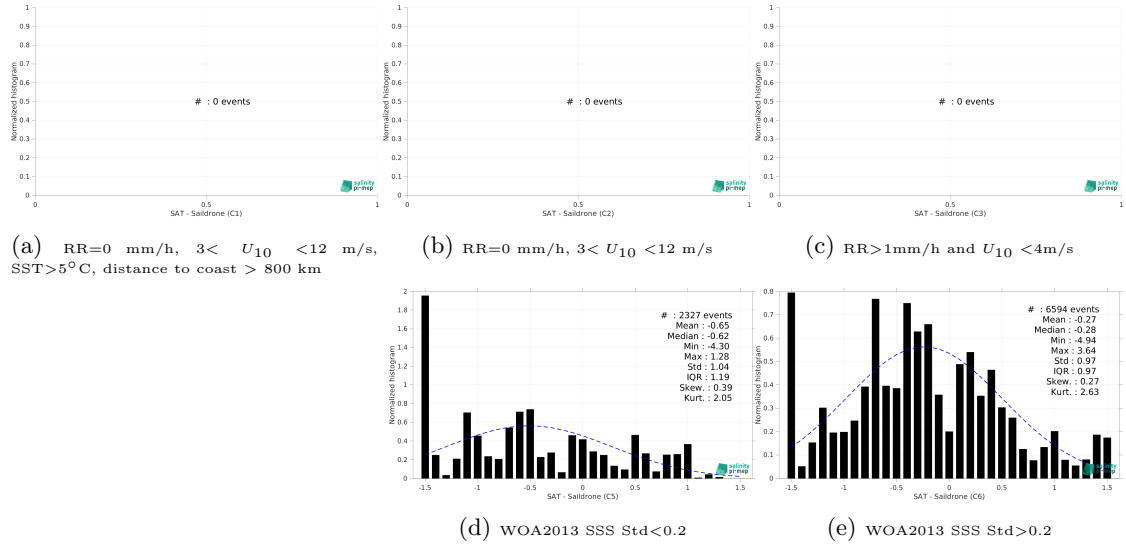
Figure 15: Normalized histogram of \Delta SSS (SMOS SSS L2Q v331 - With FLAG (CMEMS-CATDS-CPDC) - Saildrone) for 5 different subdatasets corresponding to: RR=0 mm/h, 3 < U_{10} < 12 m/s, SST>5°C, distance to coast > 800 km (a), RR=0 mm/h, 3 < U_{10} < 12 m/s (b), RR>1mm/h and U_{10} < 4 m/s (c), WOA2013 SSS Std<0.2 (d), WOA2013 SSS Std>0.2 (e).
