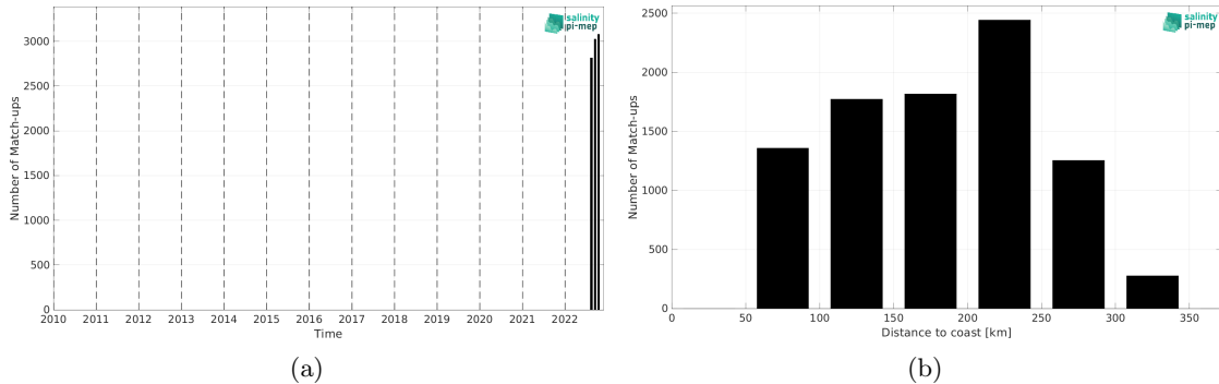
Figure 2: Number of match-ups between Saildrone and SMOS SSS L2Q v331 - With FLAG (CMEMS-CATDS-CPDC) SSS as a function of time (a) and as function of the distance to coast (b) over the Mississippi river plume Pi-MEP region and for the full satellite product period.
