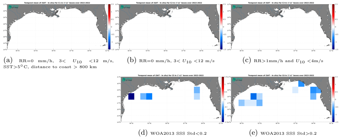
Figure 14: Temporal mean gridded over spatial boxes of size 1^\circ \times 1^\circ of \Delta\text{SSS} (SMOS SSS L2Q v331 - With FLAG (CMEMS-CATDS-CPDC) - Saildrone) for 5 different subdatasets corresponding to: RR=0 mm/h, 3 < U_{10} < 12 m/s, SST > 5°C, distance to coast > 800 km (a), RR=0 mm/h, 3 < U_{10} < 12 m/s (b), RR > 1mm/h and U_{10} < 4 m/s (c), WOA2013 SSS Std < 0.2 (d), WOA2013 SSS Std > 0.2 (e).
