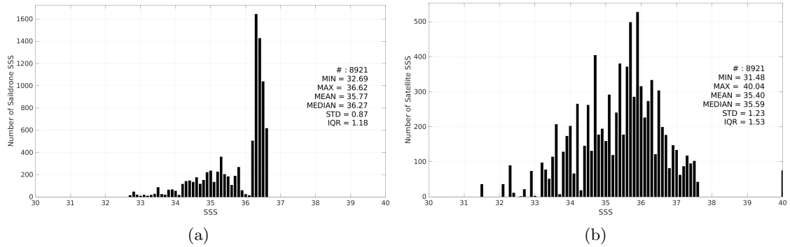
Figure 3: Histograms of SSS from Saildrone (a) and SMOS SSS L2Q v331 - With FLAG (CMEMS-CATDS-CPDC) (b) considering all match-up pairs per bins of 0.1 over the Mississippi river plume Pi-MEP region and for the full satellite product period.
