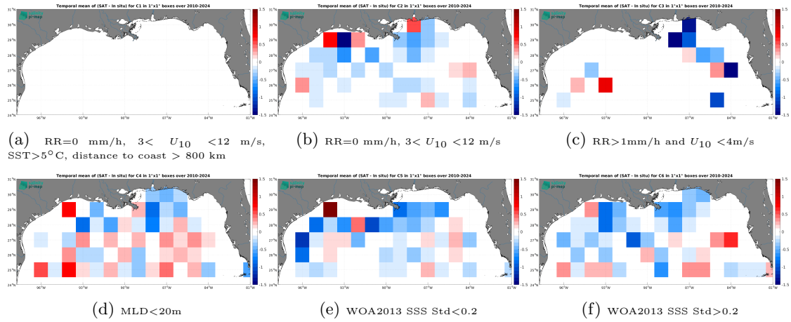
Figure 14: Temporal mean gridded over spatial boxes of size 1^\circ \times 1^\circ of \Delta SSS (SMOS SSS L2Q v331 - With FLAG (CMEMS-CATDS-CPDC) - Argo) for 6 different subdatasets corresponding to:RR=0 mm/h, 3 < U_{10} < 12 m/s, SST >5^\circ C, distance to coast > 800 km (a), RR=0 mm/h, 3 < U_{10} < 12 m/s (b), RR >1 mm/h and U_{10} < 4 m/s (c),MLD <20 m (d),WOA2013 SSS Std <0.2 (e),WOA2013 SSS Std >0.2 (f).
