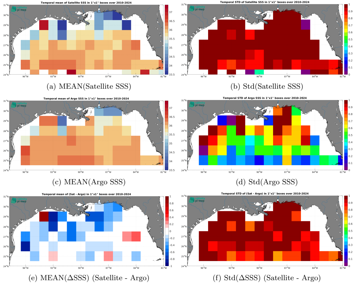
Figure 7: Temporal mean (left) and Std (right) of SSS from SMOS SSS L2Q v331 - With FLAG (CMEMS-CATDS-CPDC) (top), Argo (middle), and of \Delta\text{SSS} (Satellite - Argo). Only match-up pairs are used to generate these maps.
