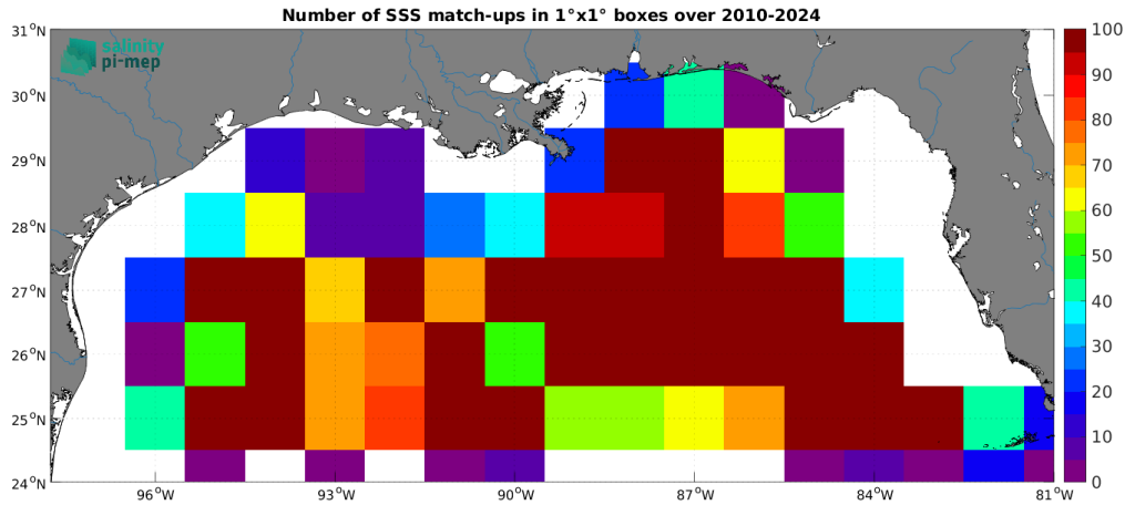
Figure 5: Number of SSS match-ups between Argo SSS and the SMOS SSS L2Q v331 - With FLAG (CMEMS-CATDS-CPDC) SSS product for the Mississippi river plume Pi-MEP region over 1^\circ \times 1^\circ boxes and for the full satellite product period.
