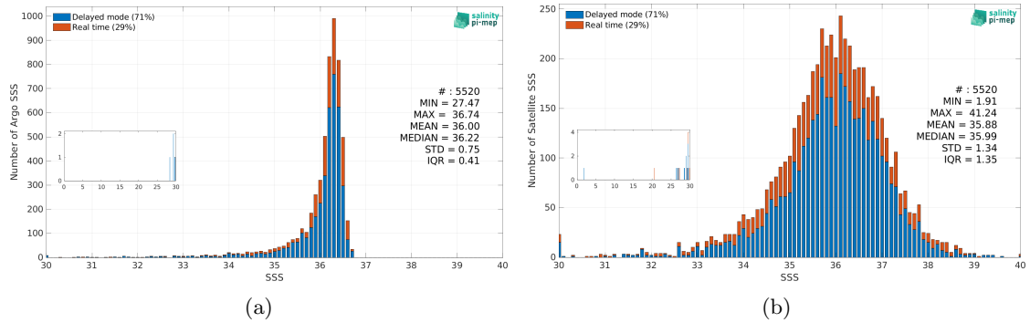
Figure 3: Histograms of SSS from Argo (a) and SMOS SSS L2Q v331 - With FLAG (CMEMS-CATDS-CPDC) (b) considering all match-up pairs per bins of 0.1 over the Mississippi river plume Pi-MEP region and for the full satellite product period.
