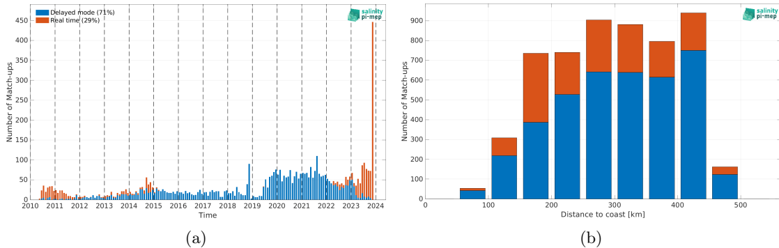
Figure 2: Number of match-ups between Argo and SMOS SSS L2Q v331 - With FLAG (CMEMS-CATDS-CPDC) SSS as a function of time (a) and as function of the distance to coast (b) over the Mississippi river plume Pi-MEP region and for the full satellite product period.
