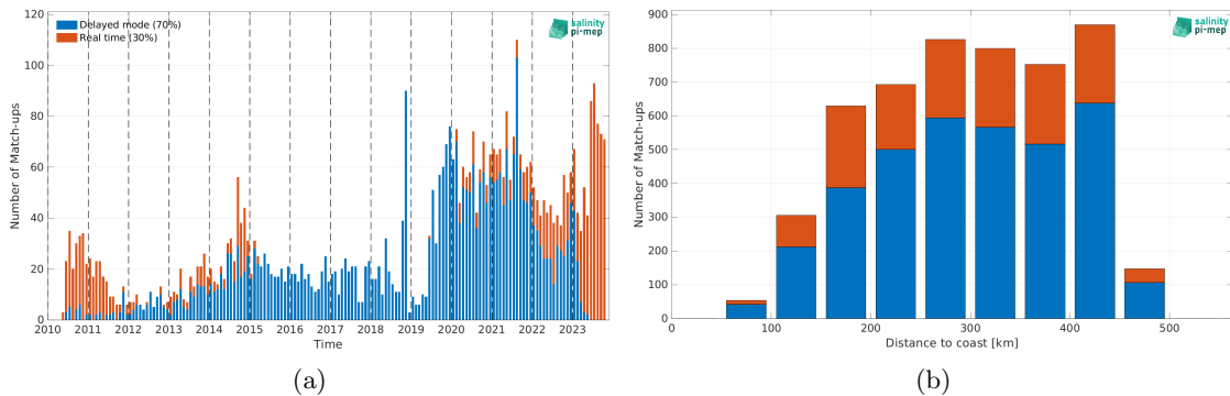
Figure 1: Number of match-ups between Argo and SMOS SSS L2Q v331 - With FLAG (CMEMS-CATDS-CPDC) SSS as a function of time (a) and as function of the distance to coast (b) over the Mississippi river plume Pi-MEP region and for the full satellite product period.
