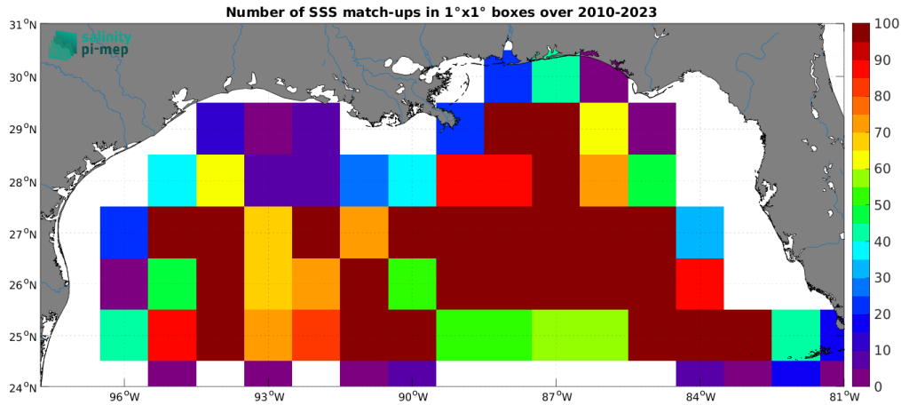
Figure 4: Number of SSS match-ups between Argo SSS and the SMOS SSS L2Q v331 - With FLAG (CMEMS-CATDS-CPDC) SSS product for the Mississippi river plume Pi-MEP region over 1^\circ \times 1^\circ boxes and for the full satellite product period.
