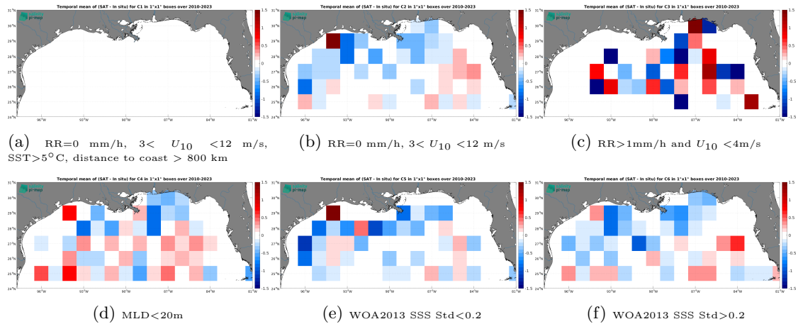
Figure 12: Temporal mean gridded over spatial boxes of size 1^{\circ}\times 1^{\circ} of \Delta\text{SSS} (SMOS SSS L2Q v331 - With FLAG (CMEMS-CATDS-CPDC) - Argo) for 6 different subdatasets corresponding to: RR=0 mm/h, 3 < U_{10} < 12 m/s, SST > 5^{\circ}\text{C} , distance to coast > 800 km (a), RR=0 mm/h, 3 < U_{10} < 12 m/s (b), RR > 1\text{mm/h} and U_{10} < 4\text{m/s} (c), MLD < 20\text{m} (d), WOA2013 SSS Std < 0.2 (e), WOA2013 SSS Std > 0.2 (f).
