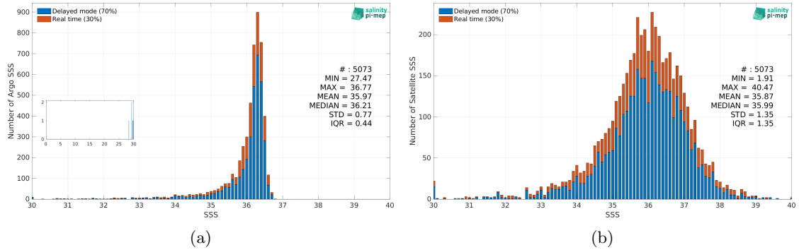
Figure 2: Histograms of SSS from Argo (a) and SMOS SSS L2Q v331 - With FLAG (CMEMS-CATDS-CPDC) (b) considering all match-up pairs per bins of 0.1 over the Mississippi river plume Pi-MEP region and for the full satellite product period.
