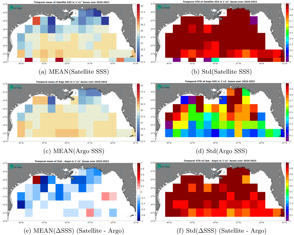
Figure 6: Temporal mean (left) and Std (right) of SSS from SMOS SSS L2Q v331 - With FLAG (CMEMS-CATDS-CPDC) (top), Argo (middle), and of \Delta\text{SSS} (Satellite - Argo). Only match-up pairs are used to generate these maps.
