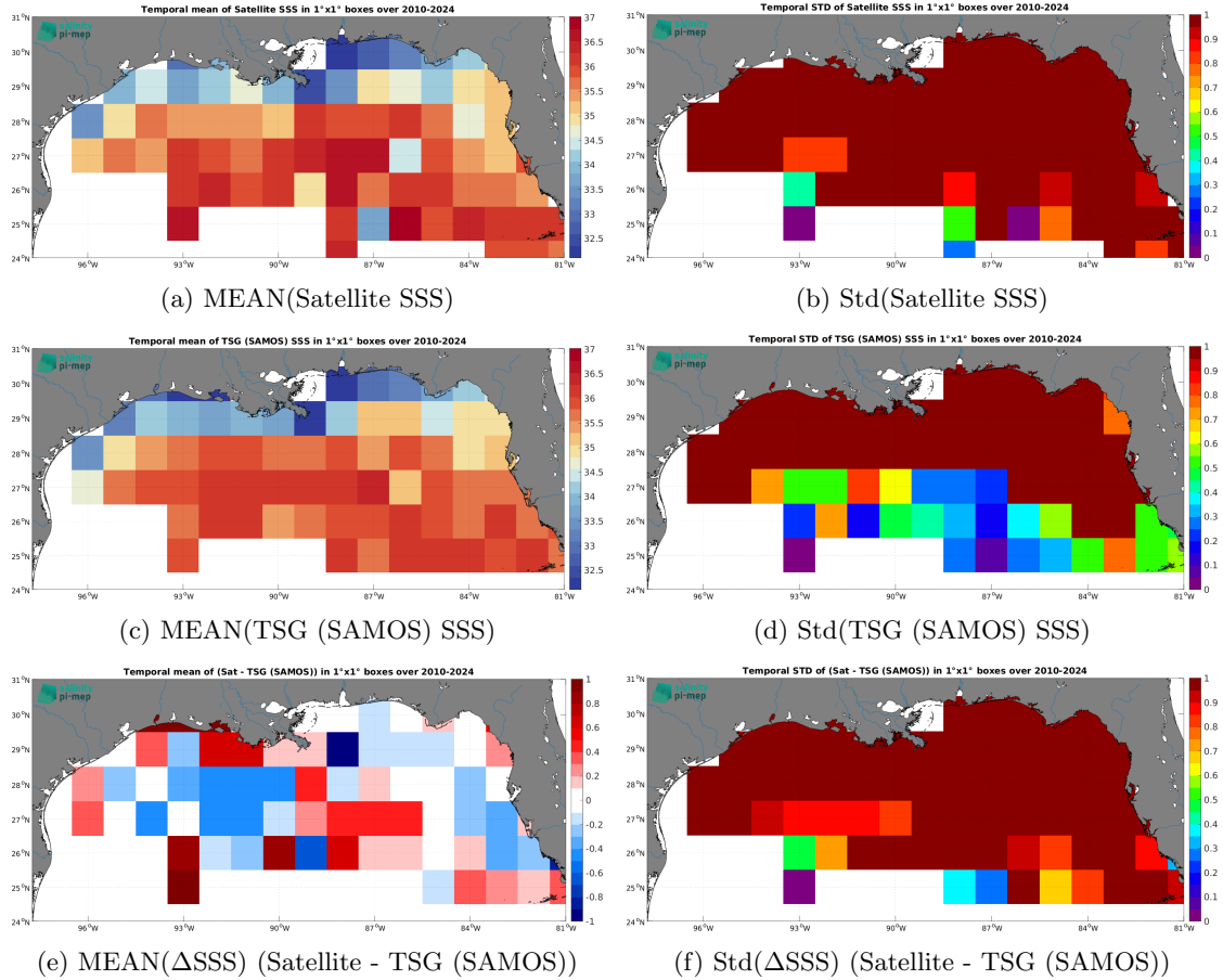
Figure 7: Temporal mean (left) and Std (right) of SSS from SMOS SSS L2Q v331 - No FLAG (CMEMS-CATDS-CPDC) (top), TSG (SAMOS) ( in situ ) (middle), and of \Delta\text{SSS} (Satellite - TSG (SAMOS)). Only match-up pairs are used to generate these maps.
