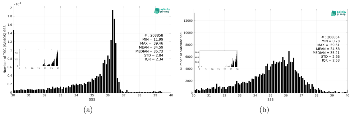
Figure 3: Histograms of SSS from TSG (SAMOS) (a) and SMOS SSS L2Q v331 - No FLAG (CMEMS-CATDS-CPDC) (b) considering all match-up pairs per bins of 0.1 over the Mississippi river plume Pi-MEP region and for the full satellite product period.
