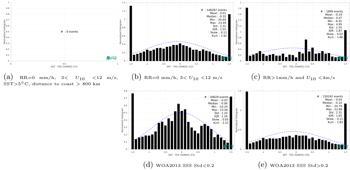
Figure 15: Normalized histogram of \Delta SSS (SMOS SSS L2Q v331 - No FLAG (CMEMS-CATDS-CPDC) - TSG (SAMOS)) for 5 different subdatasets corresponding to: RR=0 mm/h, 3 < U_{10} < 12 m/s, SST > 5°C, distance to coast > 800 km (a), RR=0 mm/h, 3 < U_{10} < 12 m/s (b), RR > 1mm/h and U_{10} < 4 m/s (c), WOA2013 SSS Std < 0.2 (d), WOA2013 SSS Std > 0.2 (e).
