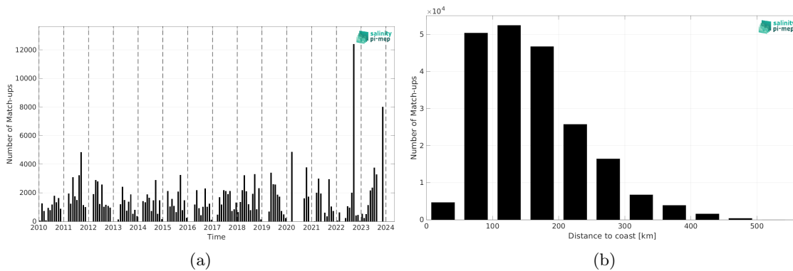
Figure 2: Number of match-ups between TSG (SAMOS) and SMOS SSS L2Q v331 - No FLAG (CMEMS-CATDS-CPDC) SSS as a function of time (a) and as function of the distance to coast (b) over the Mississippi river plume Pi-MEP region and for the full satellite product period.
