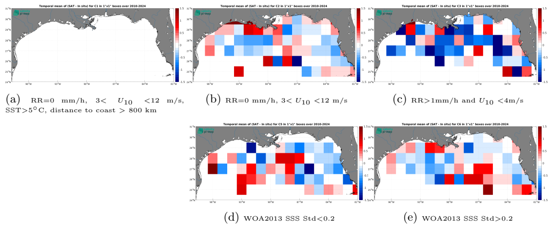
Figure 14: Temporal mean gridded over spatial boxes of size 1^\circ \times 1^\circ of \Delta SSS (SMOS SSS L2Q v331 - No FLAG (CMEMS-CATDS-CPDC) - TSG (SAMOS)) for 5 different subdatasets corresponding to: RR=0 mm/h, 3 < U_{10} < 12 m/s, SST > 5°C, distance to coast > 800 km (a), RR=0 mm/h, 3 < U_{10} < 12 m/s (b), RR > 1mm/h and U_{10} < 4 m/s (c), WOA2013 SSS Std < 0.2 (d), WOA2013 SSS Std > 0.2 (e).
