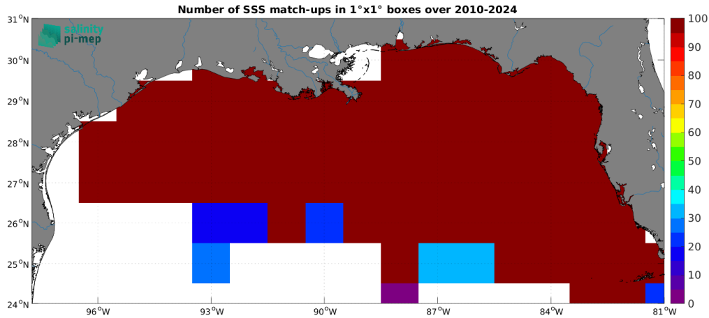
Figure 5: Number of SSS match-ups between TSG (SAMOS) SSS and the SMOS SSS L2Q v331 - No FLAG (CMEMS-CATDS-CPDC) SSS product for the Mississippi river plume Pi-MEP region over 1^\circ \times 1^\circ boxes and for the full satellite product period.
