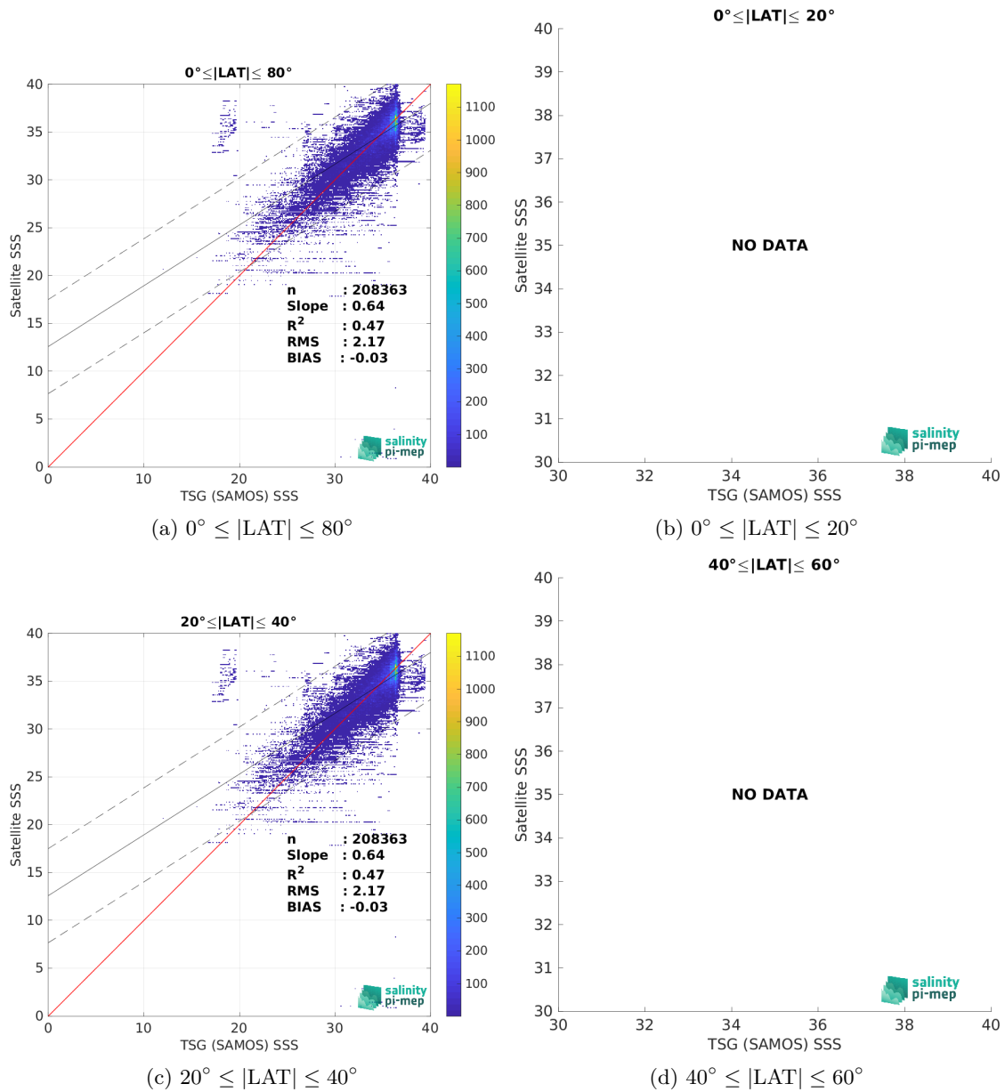
Figure 10: Contour maps of the concentration of SMOS SSS L2Q v331 - No FLAG (CMEMS-CATDS-CPDC) SSS (y-axis) versus TSG (SAMOS) SSS (x-axis) at match-up pairs for different latitude bands. For each plot, the red line shows x=y . The black thin and dashed lines indicate a linear fit through the data cloud and the \pm 95\% confidence levels, respectively. The number match-up pairs n , the slope and R^2 coefficient of the linear fit, the root mean square (RMS) and the mean bias between satellite and in situ data are indicated for each latitude band in each plots.
