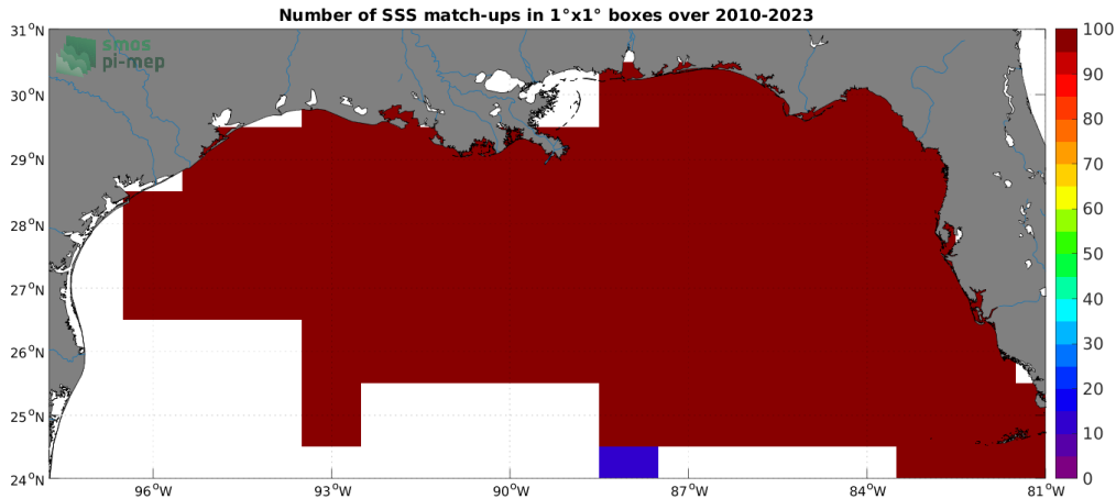
Figure 4: Number of SSS match-ups between TSG (SAMOS) SSS and the SMOS SSS L2Q v331 - No FLAG (CMEMS-CATDS-CPDC) SSS product for the Mississippi river plume Pi-MEP region over 1^\circ \times 1^\circ boxes and for the full satellite product period.
