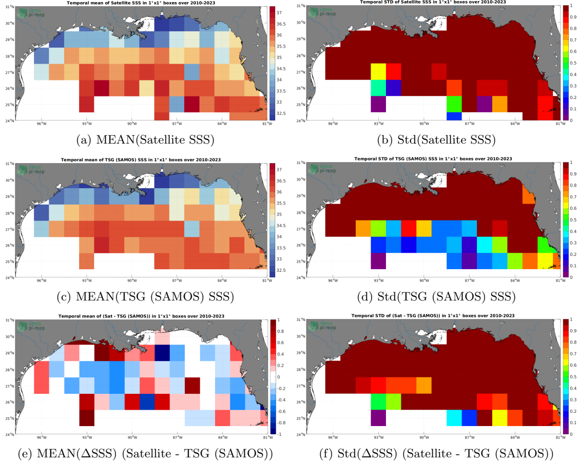
Figure 6: Temporal mean (left) and Std (right) of SSS from SMOS SSS L2Q v331 - No FLAG (CMEMS-CATDS-CPDC) (top), TSG (SAMOS) (middle), and of \Delta\text{SSS} (Satellite - TSG (SAMOS)). Only match-up pairs are used to generate these maps.
