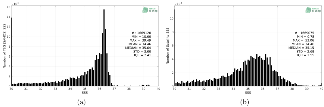
Figure 2: Histograms of SSS from TSG (SAMOS) (a) and SMOS SSS L2Q v331 - No FLAG (CMEMS-CATDS-CPDC) (b) considering all match-up pairs per bins of 0.1 over the Mississippi river plume Pi-MEP region and for the full satellite product period.
