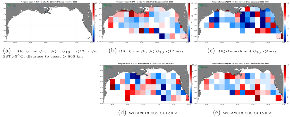
Figure 12: Temporal mean gridded over spatial boxes of size 1^{\circ}\times 1^{\circ} of \Delta\text{SSS} (SMOS SSS L2Q v331 - No FLAG (CMEMS-CATDS-CPDC) - TSG (SAMOS)) for 5 different subdatasets corresponding to:RR=0 mm/h, 3 < U_{10} < 12 m/s, SST >5^{\circ}\text{C} , distance to coast > 800 km (a), RR=0 mm/h, 3 < U_{10} < 12 m/s (b), RR >1 mm/h and U_{10} < 4 m/s (c), WOA2013 SSS Std <0.2 (d), WOA2013 SSS Std >0.2 (e).
