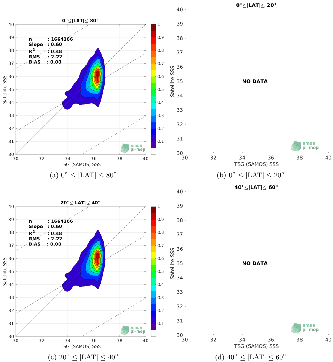
Figure 9: Contour maps of the concentration of SMOS SSS L2Q v331 - No FLAG (CMEMS-CATDS-CPDC) SSS (y-axis) versus TSG (SAMOS) SSS (x-axis) at match-up pairs for different latitude bands. For each plot, the red line shows x=y . The black thin and dashed lines indicate a linear fit through the data cloud and the \pm 95\% confidence levels, respectively. The number match-up pairs n , the slope and R^2 coefficient of the linear fit, the root mean square (RMS) and the mean bias between satellite and in situ data are indicated for each latitude band in each plots.
