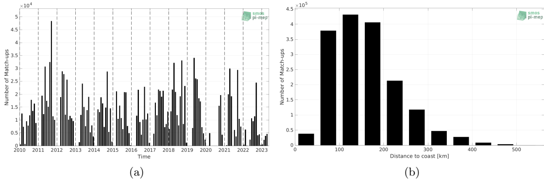
Figure 1: Number of match-ups between TSG (SAMOS) and SMOS SSS L2Q v331 - No FLAG (CMEMS-CATDS-CPDC) SSS as a function of time (a) and as function of the distance to coast (b) over the Mississippi river plume Pi-MEP region and for the full satellite product period.
