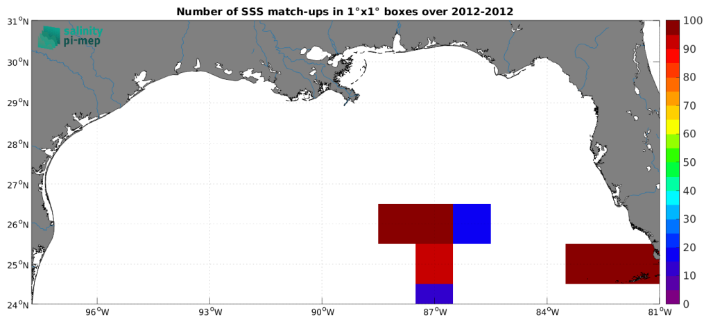
Figure 5: Number of SSS match-ups between TSG (GOSUD-Sailing-ship) SSS and the SMOS SSS L2Q v331 - No FLAG (CMEMS-CATDS-CPDC) SSS product for the Mississippi river plume Pi-MEP region over 1^\circ \times 1^\circ boxes and for the full satellite product period.
