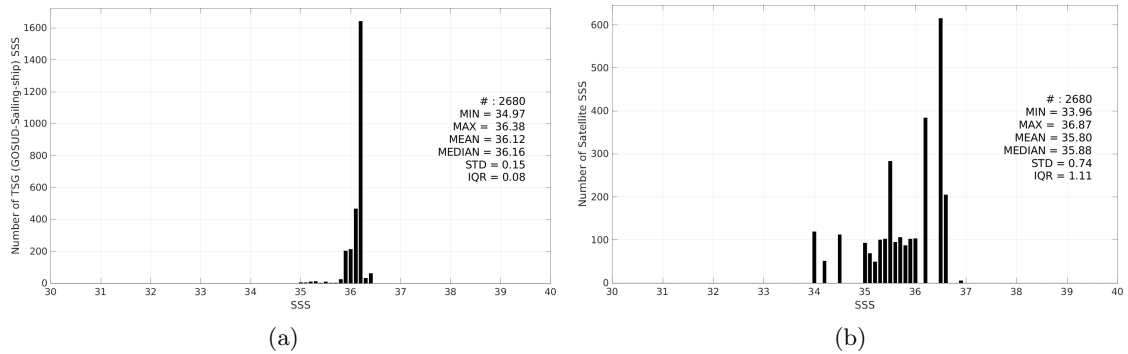
Figure 3: Histograms of SSS from TSG (GOSUD-Sailing-ship) (a) and SMOS SSS L2Q v331 - No FLAG (CMEMS-CATDS-CPDC) (b) considering all match-up pairs per bins of 0.1 over the Mississippi river plume Pi-MEP region and for the full satellite product period.
