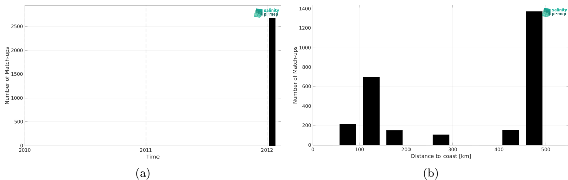
Figure 2: Number of match-ups between TSG (GOSUD-Sailing-ship) and SMOS SSS L2Q v331 - No FLAG (CMEMS-CATDS-CPDC) SSS as a function of time (a) and as function of the distance to coast (b) over the Mississippi river plume Pi-MEP region and for the full satellite product period.
