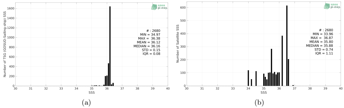
Figure 2: Histograms of SSS from TSG (GOSUD-Sailing-ship) (a) and SMOS SSS L2Q v331 - No FLAG (CMEMS-CATDS-CPDC) (b) considering all match-up pairs per bins of 0.1 over the Mississippi river plume Pi-MEP region and for the full satellite product period.
