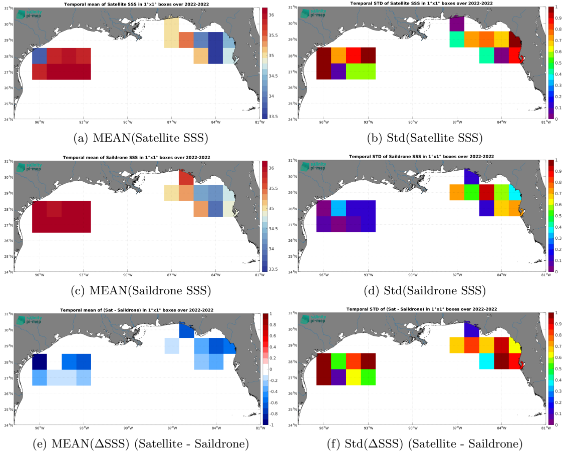
Figure 7: Temporal mean (left) and Std (right) of SSS from SMOS SSS L2Q v331 - No FLAG (CMEMS-CATDS-CPDC) (top), Sairdrone (middle), and of \Delta SSS (Satellite - Sairdrone). Only match-up pairs are used to generate these maps.
