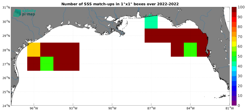
Figure 5: Number of SSS match-ups between Saildrone SSS and the SMOS SSS L2Q v331 - No FLAG (CMEMS-CATDS-CPDC) SSS product for the Mississippi river plume Pi-MEP region over 1^\circ \times 1^\circ boxes and for the full satellite product period.
