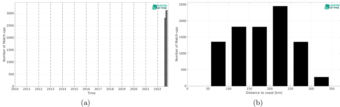
Figure 2: Number of match-ups between Saildrone and SMOS SSS L2Q v331 - No FLAG (CMEMS-CATDS-CPDC) SSS as a function of time (a) and as function of the distance to coast (b) over the Mississippi river plume Pi-MEP region and for the full satellite product period.
