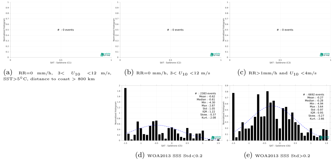
Figure 15: Normalized histogram of \Delta SSS (SMOS SSS L2Q v331 - No FLAG (CMEMS-CATDS-CPDC) - Salldrone) for 5 different subdatasets corresponding to: RR=0 mm/h, 3 < U_{10} < 12 m/s, SST>5°C, distance to coast > 800 km (a), RR=0 mm/h, 3 < U_{10} < 12 m/s (b), RR>1mm/h and U_{10} < 4 m/s (c), WOA2013 SSS Std<0.2 (d), WOA2013 SSS Std>0.2 (e).
