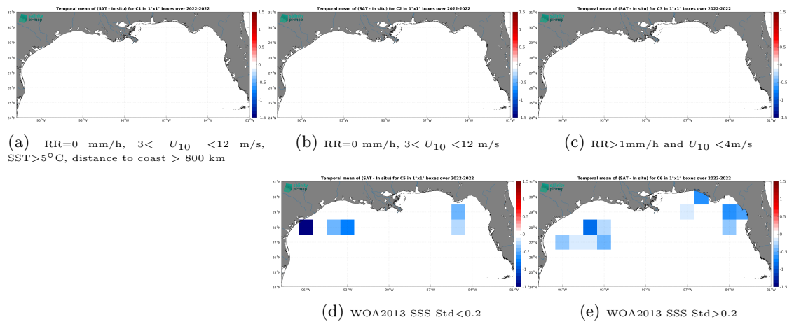
Figure 14: Temporal mean gridded over spatial boxes of size 1^\circ \times 1^\circ of \Delta SSS (SMOS SSS L2Q v331 - No FLAG (CMEMS-CATDS-CPDC) - Saildrone) for 5 different subdatasets corresponding to: RR=0 mm/h, 3 < U_{10} < 12 m/s, SST > 5°C, distance to coast > 800 km (a), RR=0 mm/h, 3 < U_{10} < 12 m/s (b), RR > 1 mm/h and U_{10} < 4 m/s (c), WOA2013 SSS Std < 0.2 (d), WOA2013 SSS Std > 0.2 (e).
