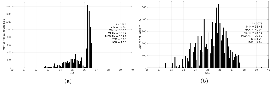
Figure 3: Histograms of SSS from Saildrone (a) and SMOS SSS L2Q v331 - No FLAG (CMEMS-CATDS-CPDC) (b) considering all match-up pairs per bins of 0.1 over the Mississippi river plume Pi-MEP region and for the full satellite product period.
