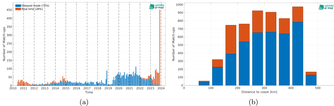
Figure 2: Number of match-ups between Argo and SMOS SSS L2Q v331 - No FLAG (CMEMS-CATDS-CPDC) SSS as a function of time (a) and as function of the distance to coast (b) over the Mississippi river plume Pi-MEP region and for the full satellite product period.
