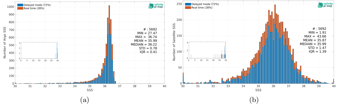
Figure 3: Histograms of SSS from Argo (a) and SMOS SSS L2Q v331 - No FLAG (CMEMS-CATDS-CPDC) (b) considering all match-up pairs per bins of 0.1 over the Mississippi river plume Pi-MEP region and for the full satellite product period.
