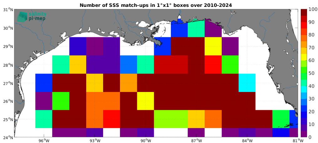
Figure 5: Number of SSS match-ups between Argo SSS and the SMOS SSS L2Q v331 - No FLAG (CMEMS-CATDS-CPDC) SSS product for the Mississippi river plume Pi-MEP region over 1^\circ \times 1^\circ boxes and for the full satellite product period.
