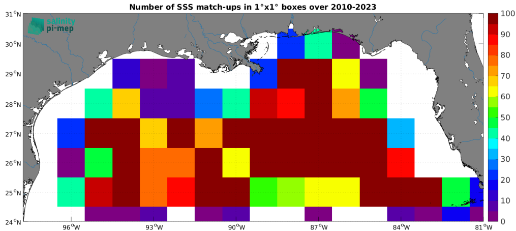
Figure 4: Number of SSS match-ups between Argo SSS and the SMOS SSS L2Q v331 - No FLAG (CMEMS-CATDS-CPDC) SSS product for the Mississippi river plume Pi-MEP region over 1^\circ \times 1^\circ boxes and for the full satellite product period.
