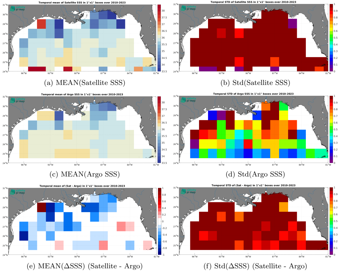
Figure 6: Temporal mean (left) and Std (right) of SSS from SMOS SSS L2Q v331 - No FLAG (CMEMS-CATDS-CPDC) (top), Argo (middle), and of \Delta\text{SSS} (Satellite - Argo). Only match-up pairs are used to generate these maps.
