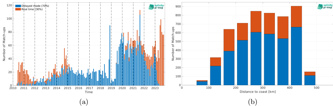
Figure 1: Number of match-ups between Argo and SMOS SSS L2Q v331 - No FLAG (CMEMS-CATDS-CPDC) SSS as a function of time (a) and as function of the distance to coast (b) over the Mississippi river plume Pi-MEP region and for the full satellite product period.
