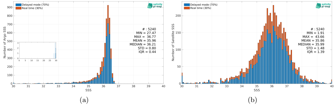
Figure 2: Histograms of SSS from Argo (a) and SMOS SSS L2Q v331 - No FLAG (CMEMS-CATDS-CPDC) (b) considering all match-up pairs per bins of 0.1 over the Mississippi river plume Pi-MEP region and for the full satellite product period.
