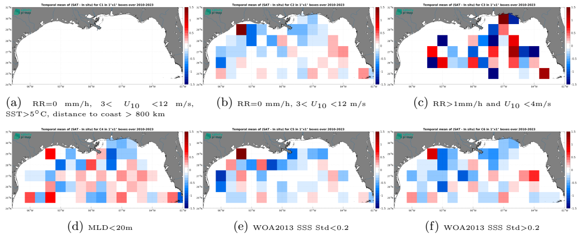
Figure 12: Temporal mean gridded over spatial boxes of size 1^{\circ}\times 1^{\circ} of \Delta\text{SSS} (SMOS SSS L2Q v331 - No FLAG (CMEMS-CATDS-CPDC) - Argo) for 6 different subdatasets corresponding to: RR=0 mm/h, 3 < U_{10} < 12 m/s, SST > 5^{\circ}\text{C} , distance to coast > 800 km (a), RR=0 mm/h, 3 < U_{10} < 12 m/s (b), RR > 1\text{mm/h} and U_{10} < 4\text{m/s} (c), MLD < 20\text{m} (d), WOA2013 SSS Std < 0.2 (e), WOA2013 SSS Std > 0.2 (f).
