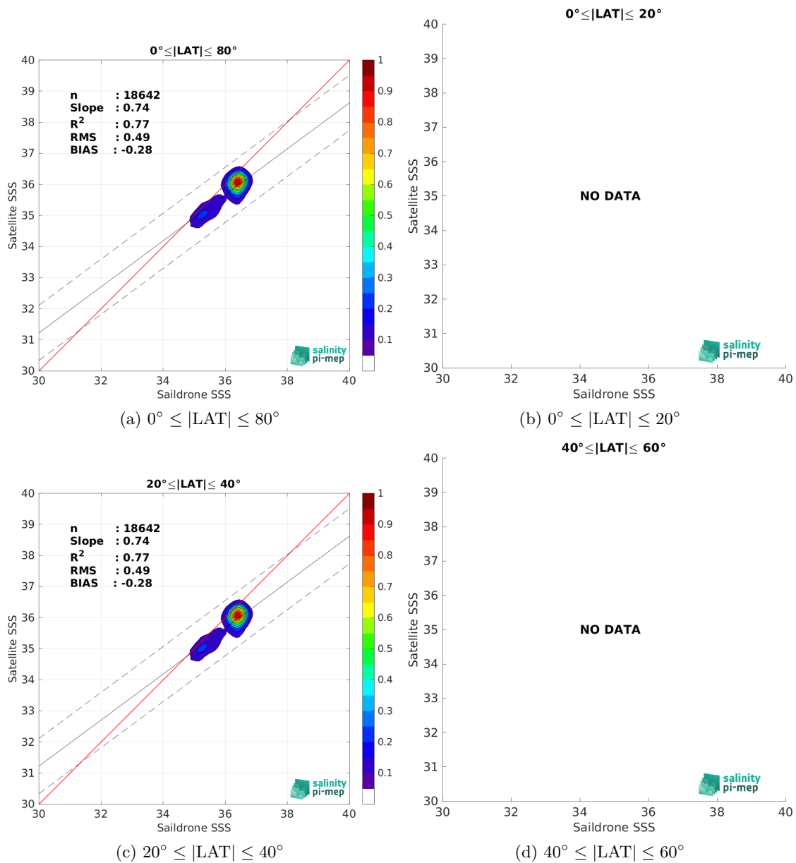
Figure 10: Contour maps of the concentration of SMOS SSS L3 v9 - 18 Days (CATDS-CEC-LOCEAN) SSS (y-axis) versus Saïldrone SSS (x-axis) at match-up pairs for different latitude bands. For each plot, the red line shows x=y . The black thin and dashed lines indicate a linear fit through the data cloud and the \pm 95\% confidence levels, respectively. The number match-up pairs n , the slope and R^2 coefficient of the linear fit, the root mean square (RMS) and the mean bias between satellite and in situ data are indicated for each latitude band in each plots.
