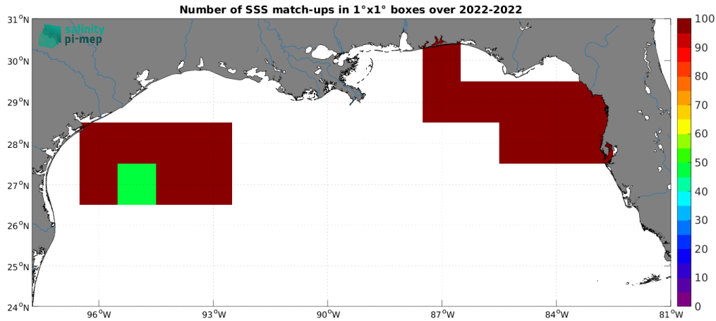
Figure 5: Number of SSS match-ups between Saildrone SSS and the SMOS SSS L3 v9 - 18 Days (CATDS-CEC-LOCEAN) SSS product for the Mississippi river plume Pi-MEP region over 1^\circ \times 1^\circ boxes and for the full satellite product period.
