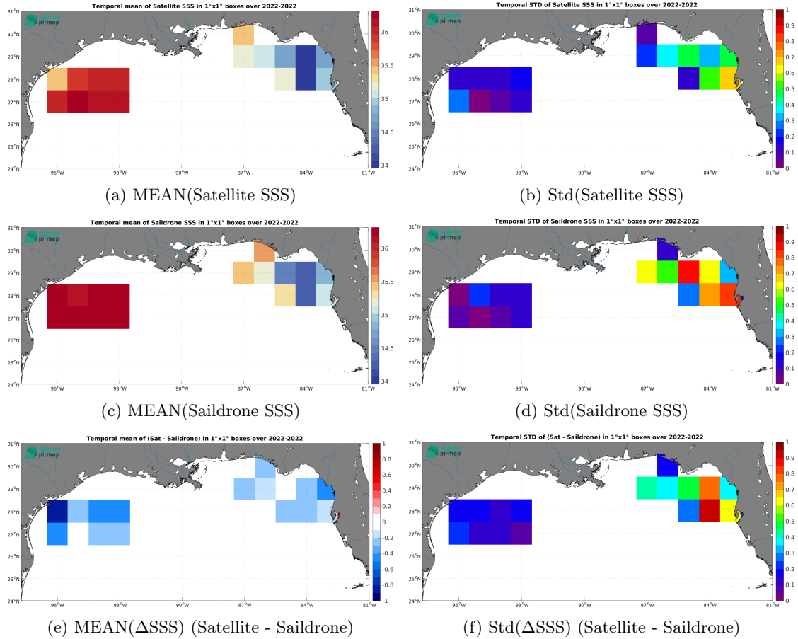
Figure 7: Temporal mean (left) and Std (right) of SSS from SMOS SSS L3 v9 - 18 Days (CATDS-CEC-LOCEAN) (top), Saildrone (middle), and of \Delta\text{SSS} (Satellite - Saildrone). Only match-up pairs are used to generate these maps.
