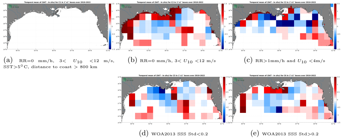
Figure 12: Temporal mean gridded over spatial boxes of size 1^{\circ}\times 1^{\circ} of \Delta\text{SSS} (SMOS SSS L3 v8 - 9 Days (CATDS-CECOS-LOCEAN) - TSG (SAMOS)) for 5 different subdatasets corresponding to:RR=0 mm/h, 3 < U_{10} < 12 m/s, SST >5^{\circ}\text{C} , distance to coast > 800 km (a), RR=0 mm/h, 3 < U_{10} < 12 m/s (b), RR >1 mm/h and U_{10} < 4 m/s (c), WOA2013 SSS Std <0.2 (d), WOA2013 SSS Std >0.2 (e).
