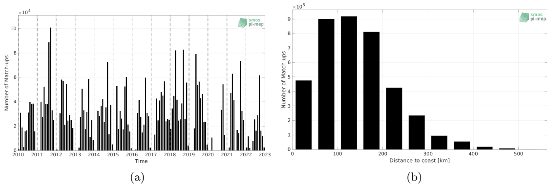
Figure 1: Number of match-ups between TSG (SAMOS) and SMOS SSS L3 v8 - 9 Days (CATDS-CECOS-LOCEAN) SSS as a function of time (a) and as function of the distance to coast (b) over the Mississippi river plume Pi-MEP region and for the full satellite product period.
