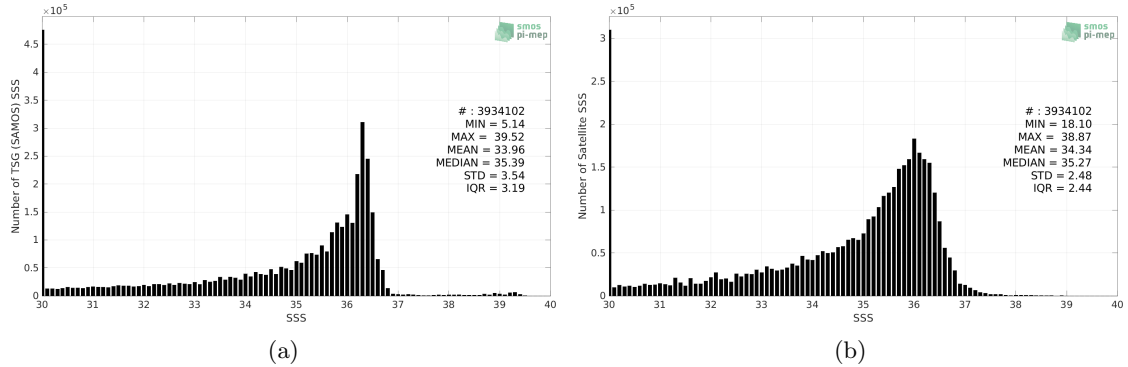
Figure 2: Histograms of SSS from TSG (SAMOS) (a) and SMOS SSS L3 v8 - 9 Days (CATDS-CECOS-LOCEAN) (b) considering all match-up pairs per bins of 0.1 over the Mississippi river plume Pi-MEP region and for the full satellite product period.
