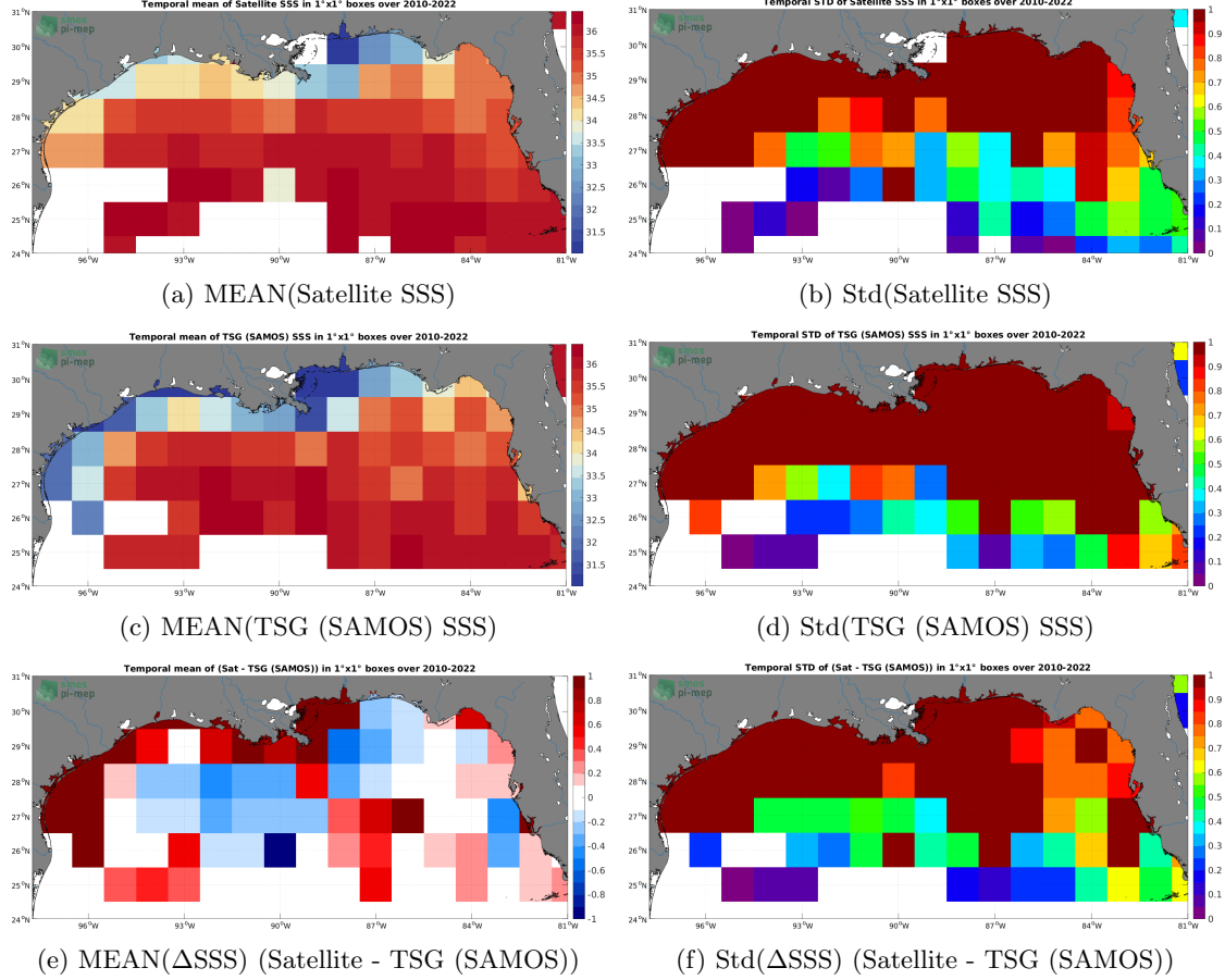
Figure 6: Temporal mean (left) and Std (right) of SSS from SMOS SSS L3 v8 - 9 Days (CATDS-CECOS-LOCEAN) (top), TSG (SAMOS) (middle), and of \Delta\text{SSS} (Satellite - TSG (SAMOS)). Only match-up pairs are used to generate these maps.
